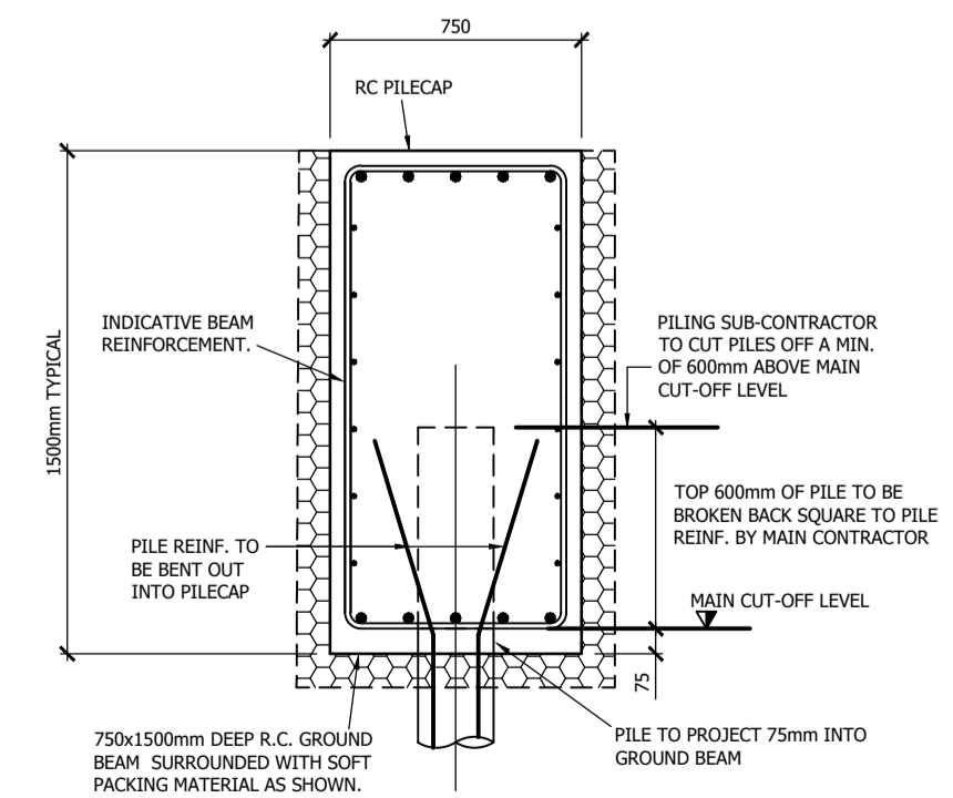
PILE CUT-OFF DETAIL (1:25)
