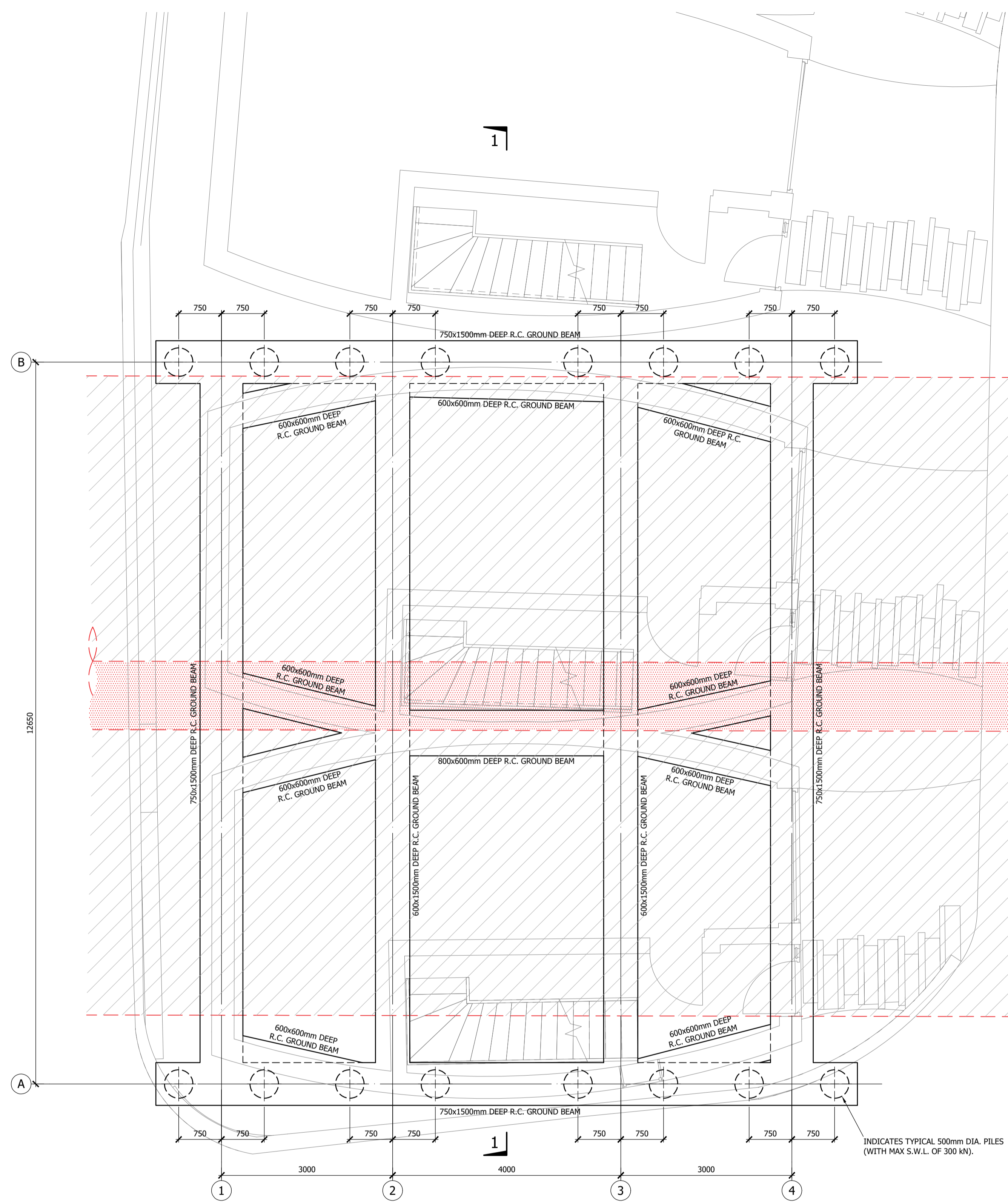
GROUND BEAM LAYOUT FOR UNITS 1 AND 2 (1:50)
