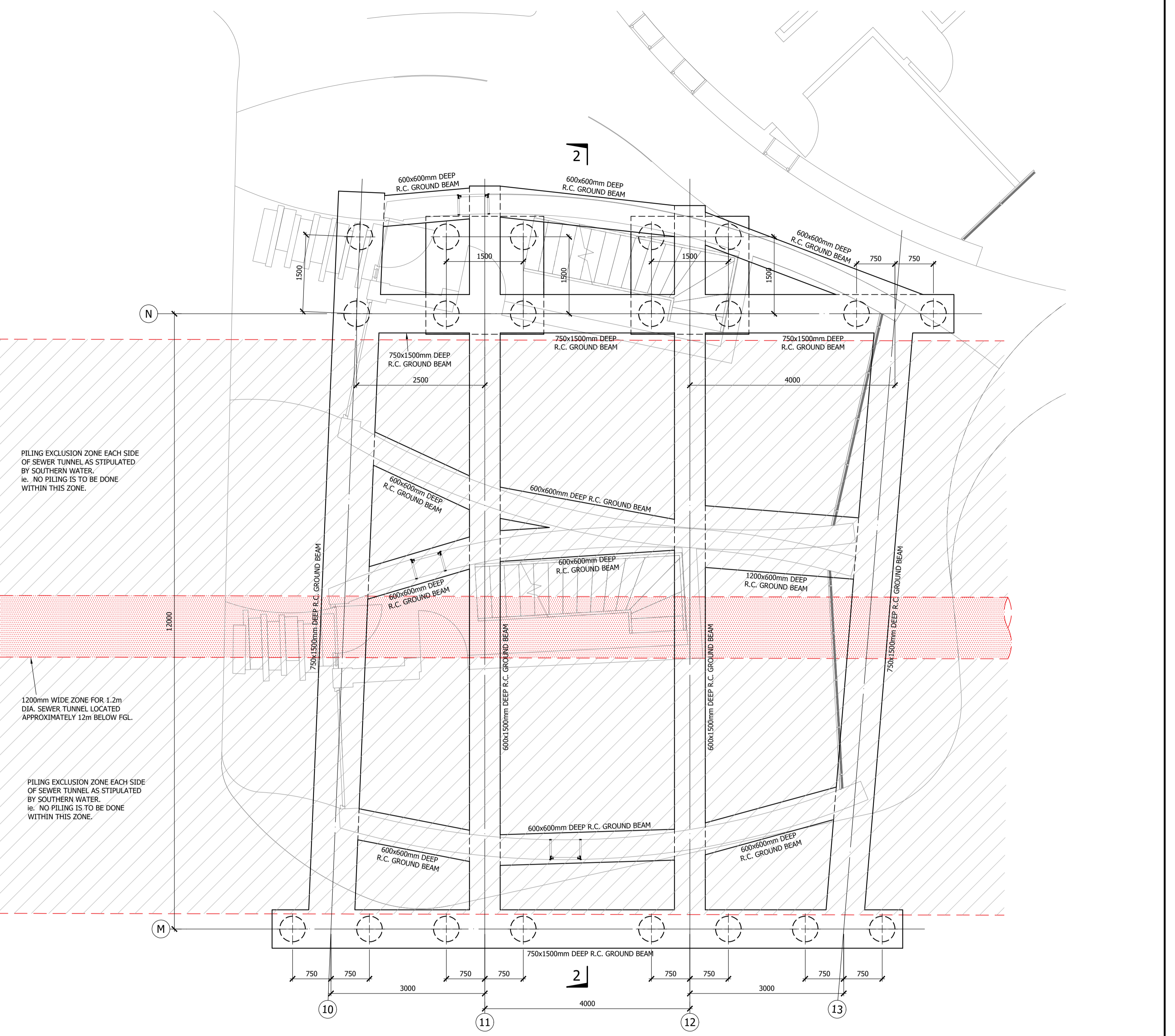
GROUND BEAM LAYOUT FOR UNITS 7 AND 8 (1:50)
