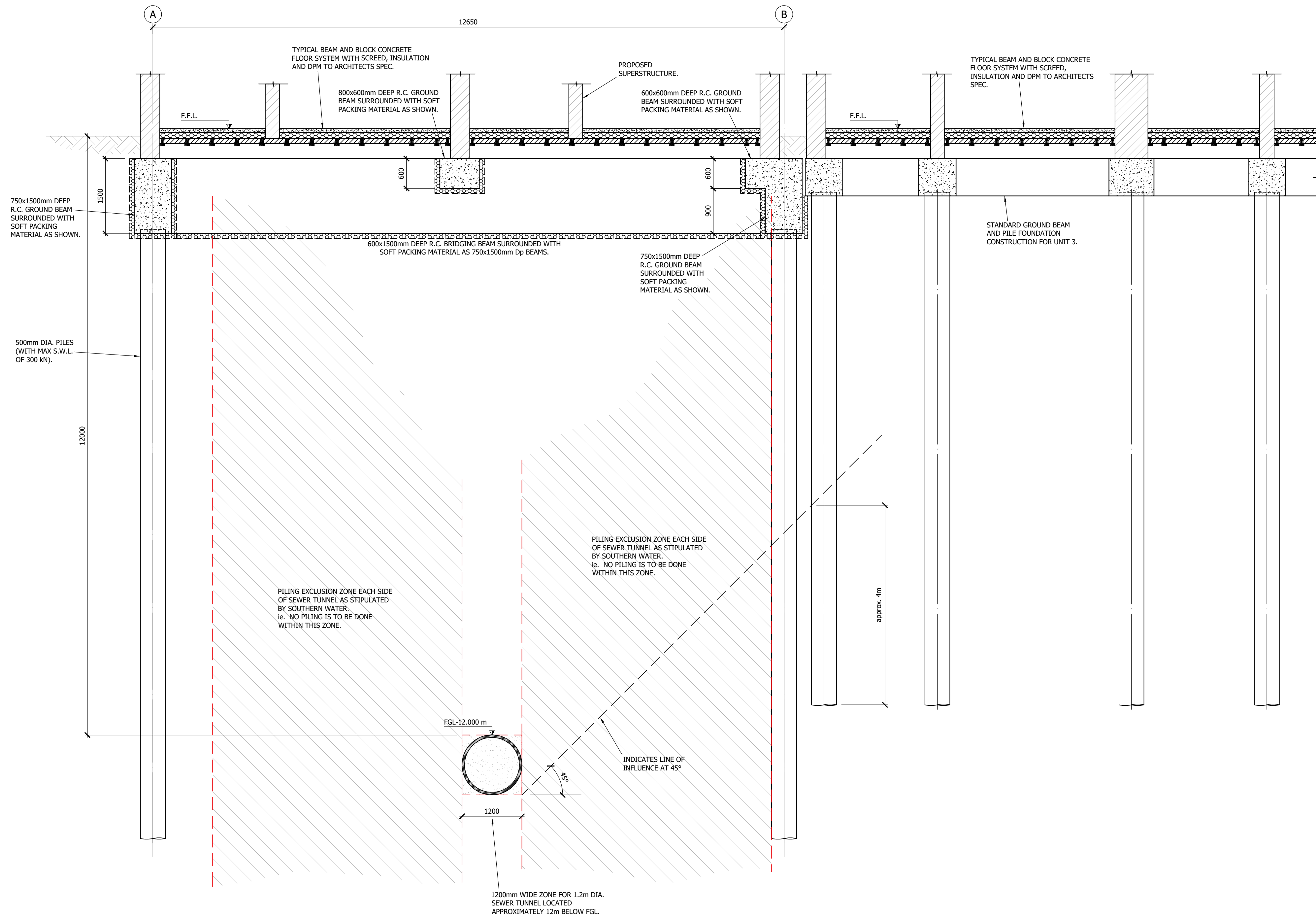
SECTION 1-1 (1:50)
