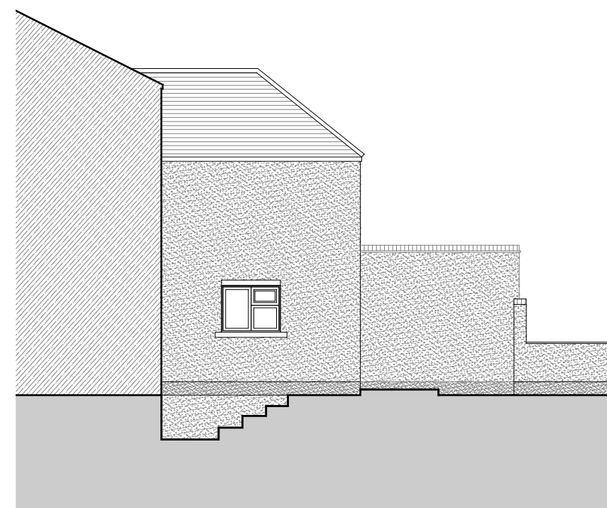
EXISTING SIDE ELEVATION 1:100 @ A3
