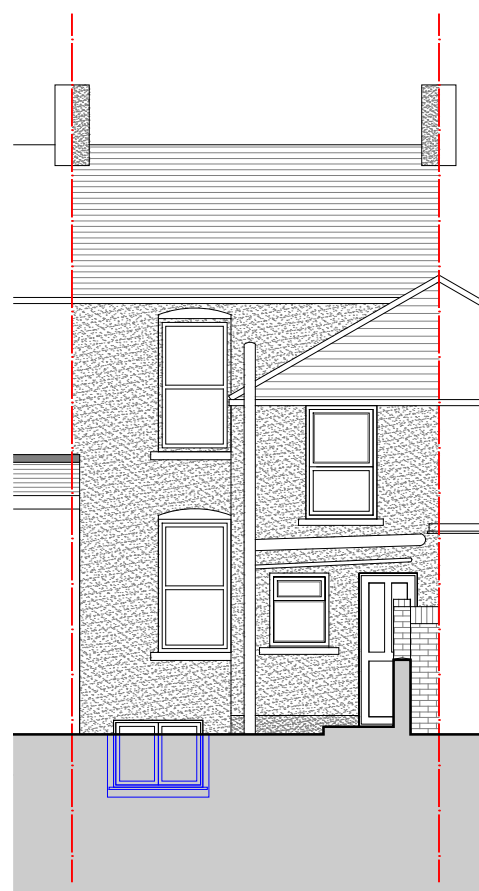
EXISTING REAR ELEVATION 1:100 @ A3
