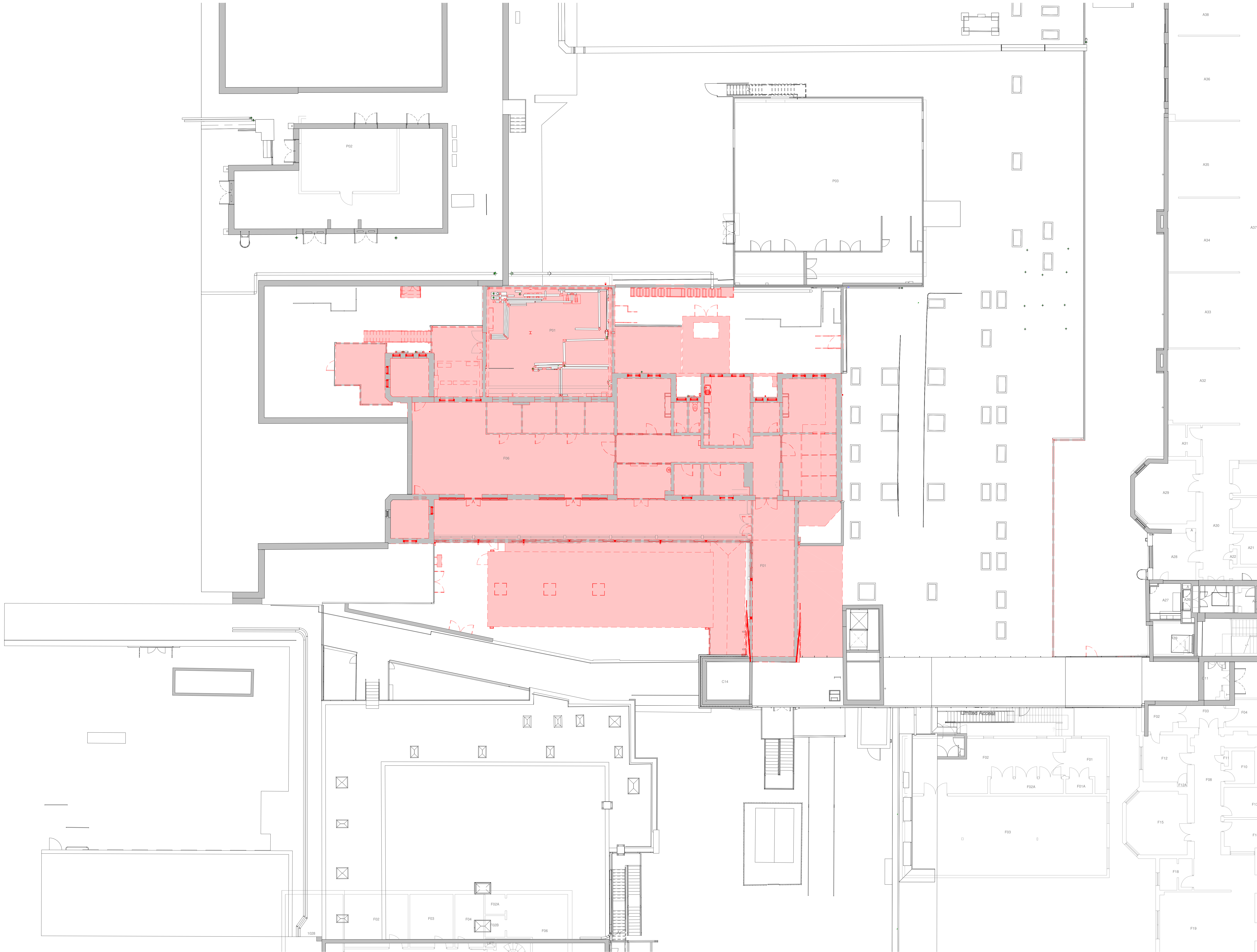
Proposed Demolition Plan First Floor 1 : 100
