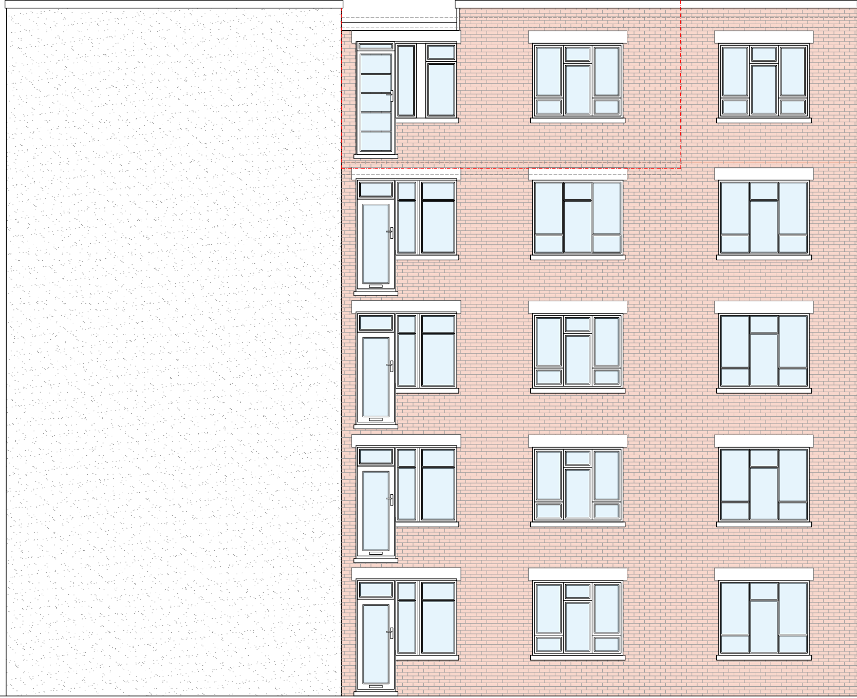
B PROPOSED REAR ELEVATION Scale: 1:75
