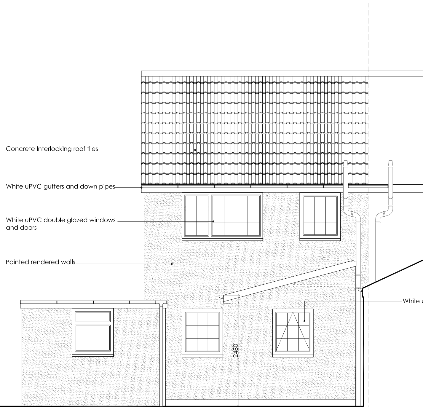
11 Beaufort Cres, Stoke Gifford Rear Elevation As Proposed (scale 1:50@A3)
