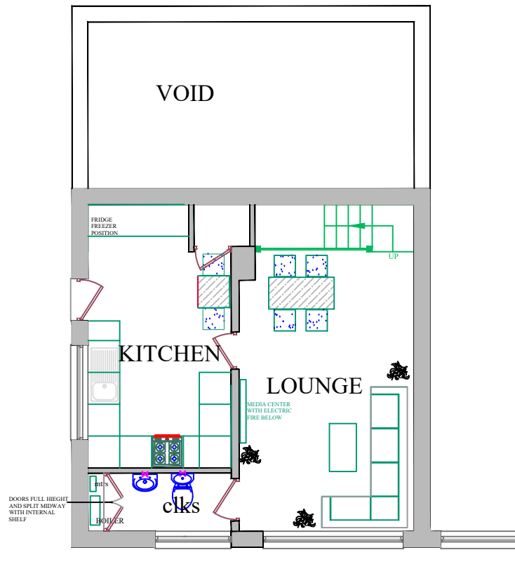
GROUND FLOOR LAYOUT TO FRONT
