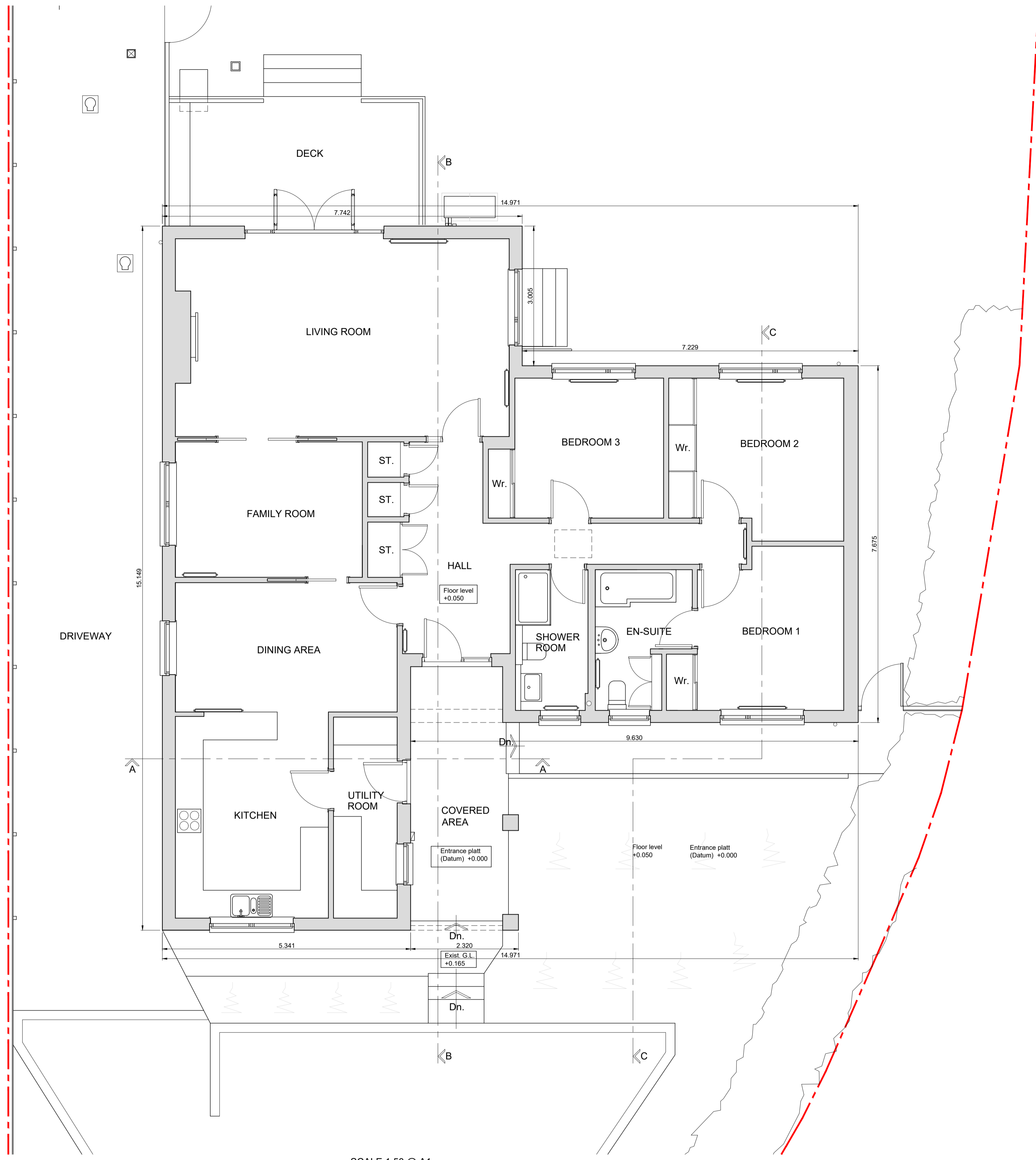
Existing Floor Plan
