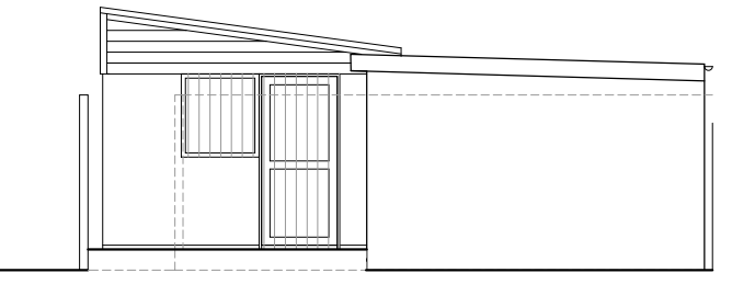
EXISTING FRONT (EAST) ELEVATION
