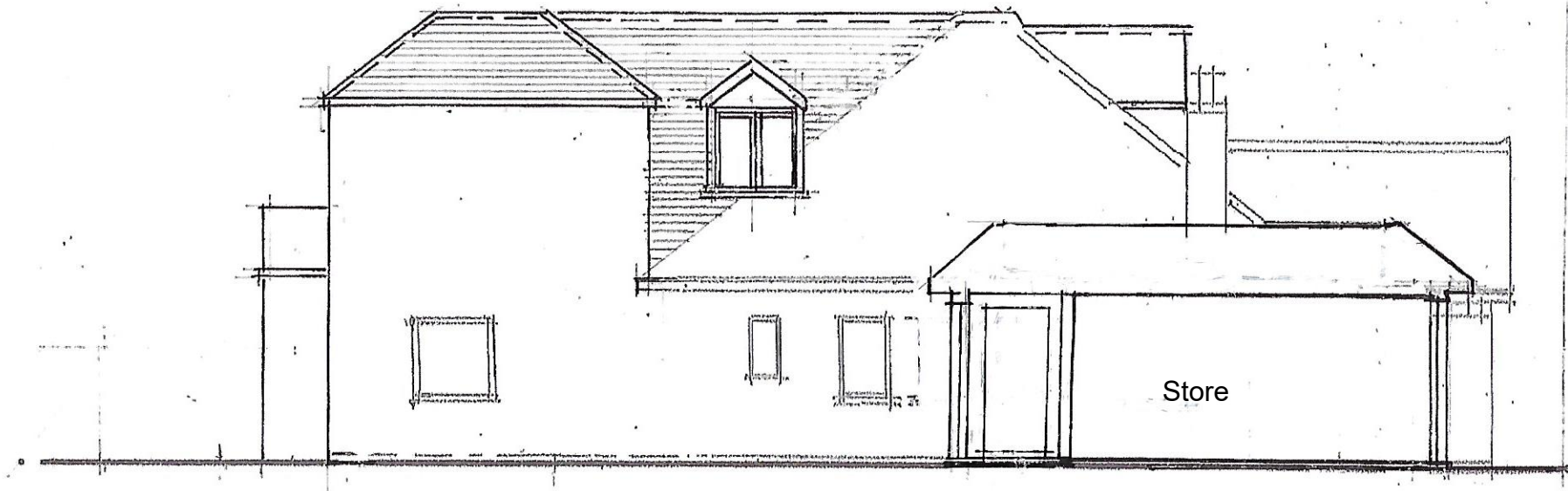
Proposed Side Elevation (East) Section
