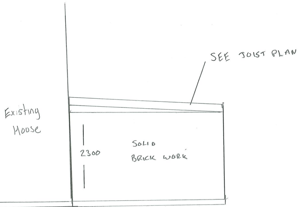
FROM REAR LEFT ELEVATION
