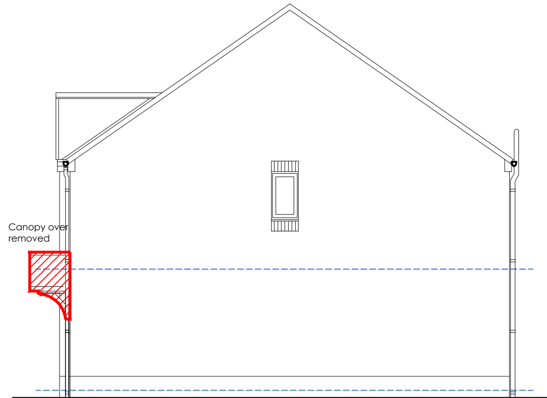
SIDE ELEVATION AS EXISTING
