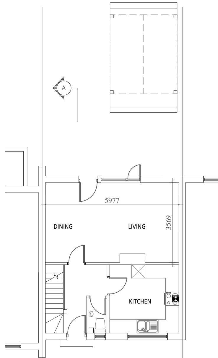
EXISTING GROUND FLOOR PLAN 7 WEST CLOSE, STEVENAGE SG1 1PW
