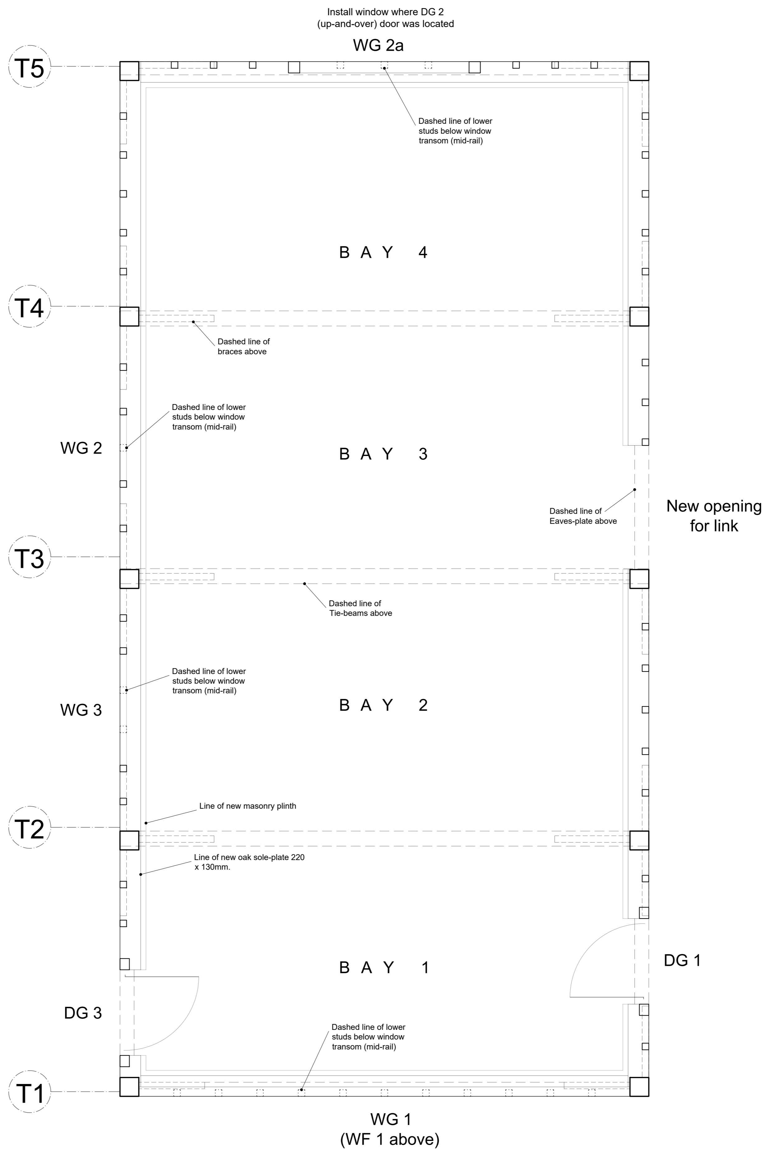
SCALE 1:25@A1 -- PROPOSED GROUND FLOOR PLAN
