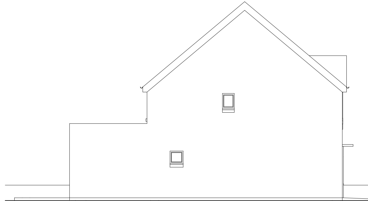
SIDE ELEVATION
