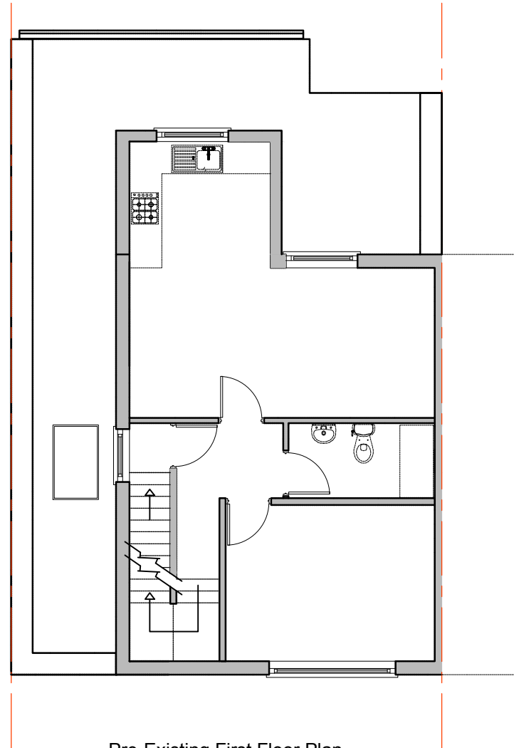
Pre-Existing First Floor Plan
