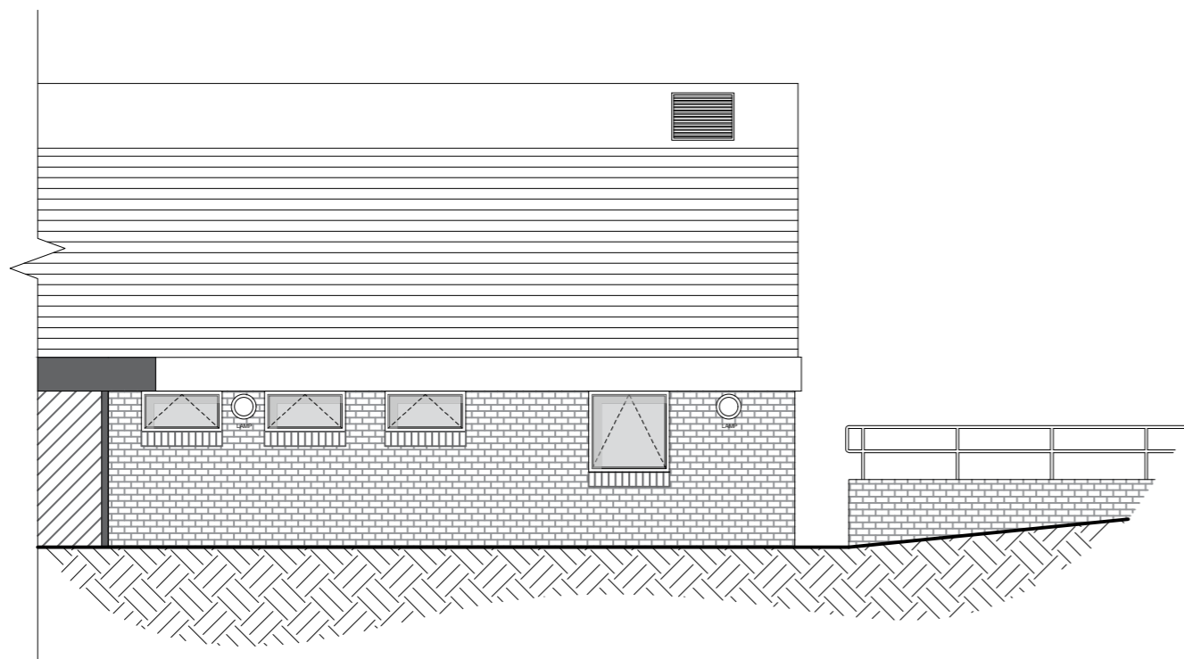
EXISTING SIDE ELEVATION (SOUTH - 01) 1:200 @ A2
