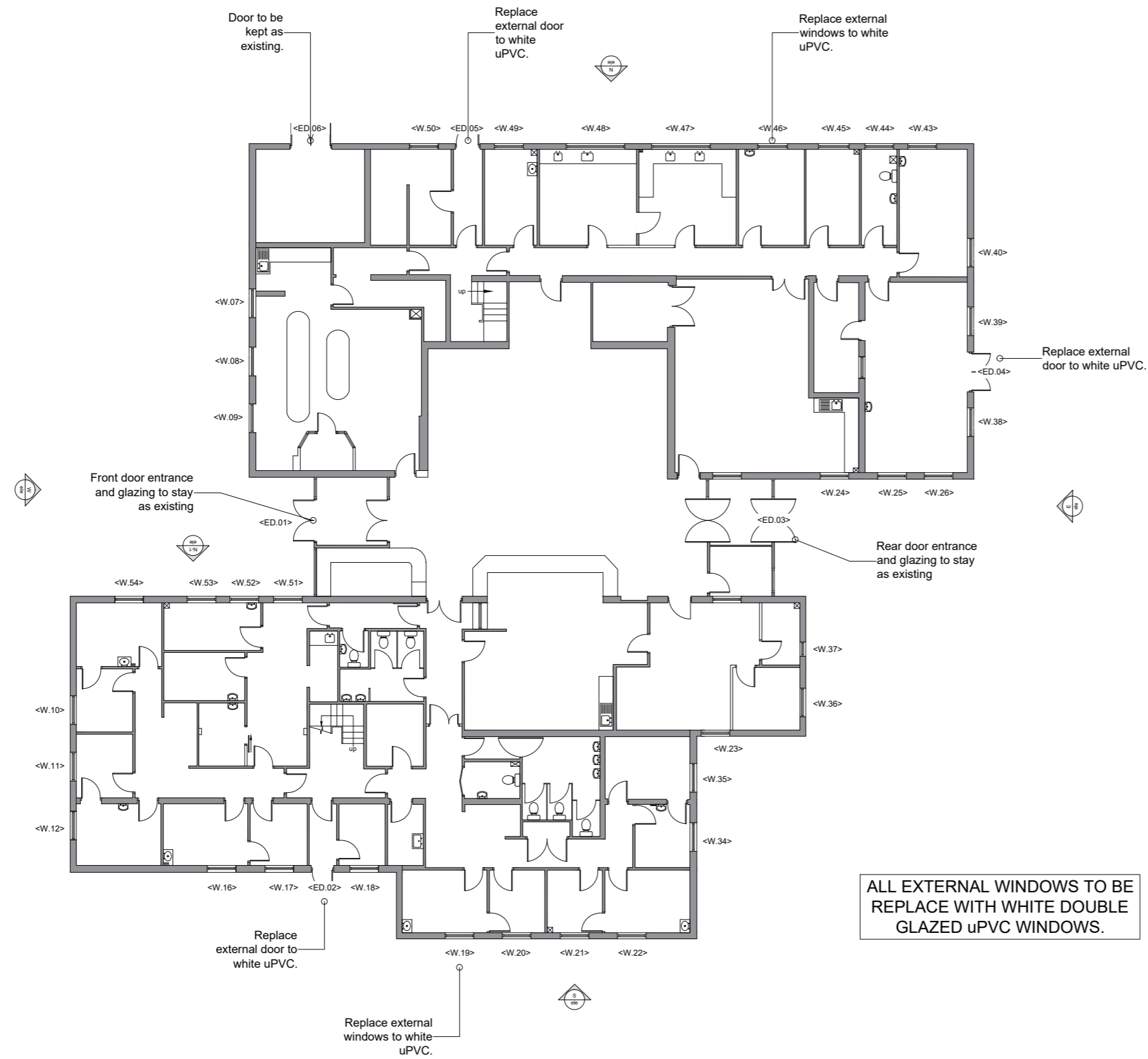
PROPOSED GROUND FLOOR PLAN 1:200 @ A2
