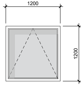
1200x1200mm Top hung window uPVC, White. (x11)
