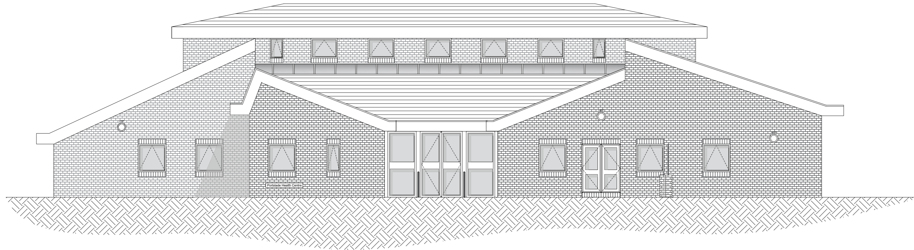
EXISTING REAR ELEVATION (EAST) 1:200 @ A2
