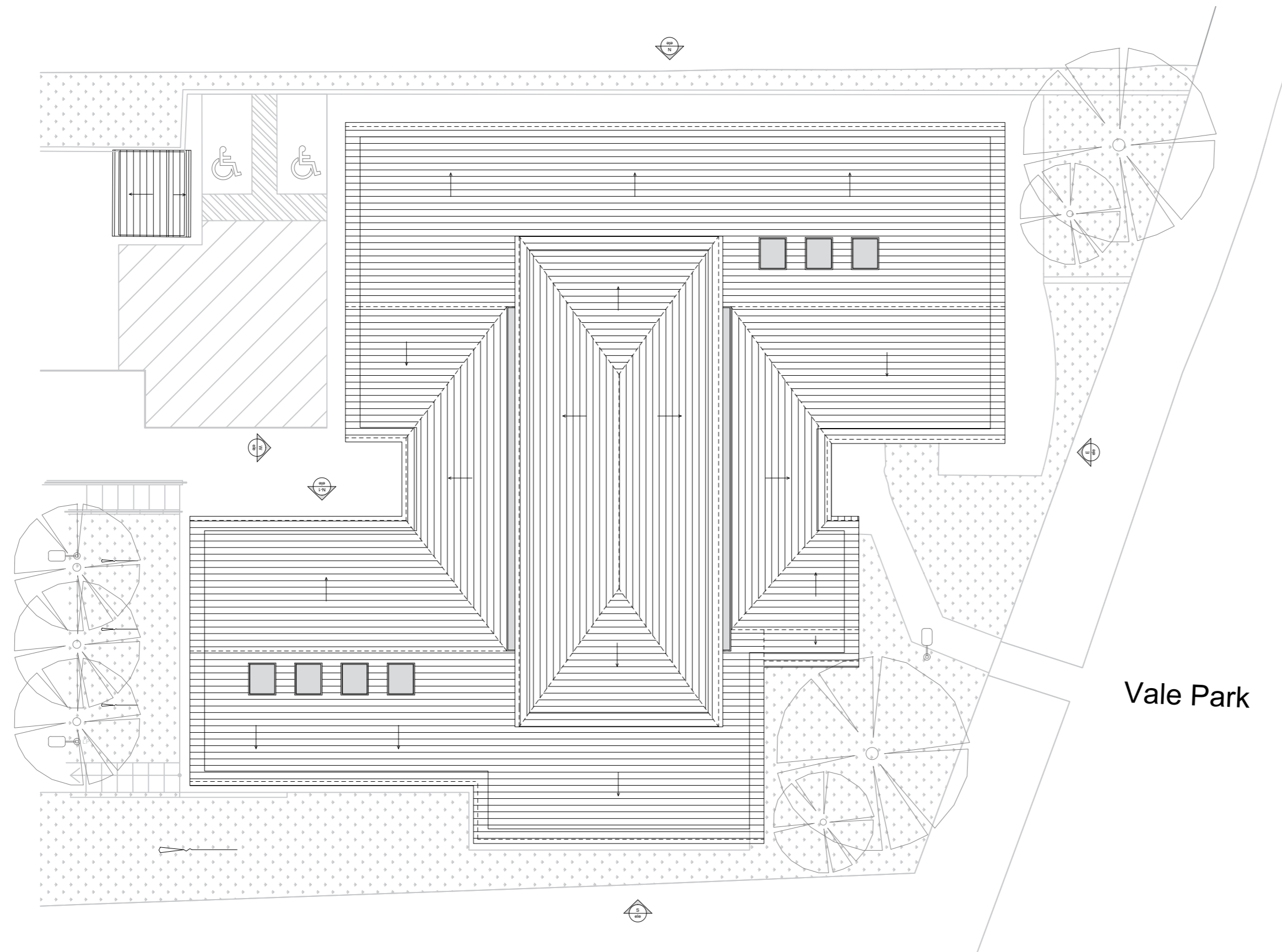
EXISTING ROOF PLAN 1:200 @ A2
