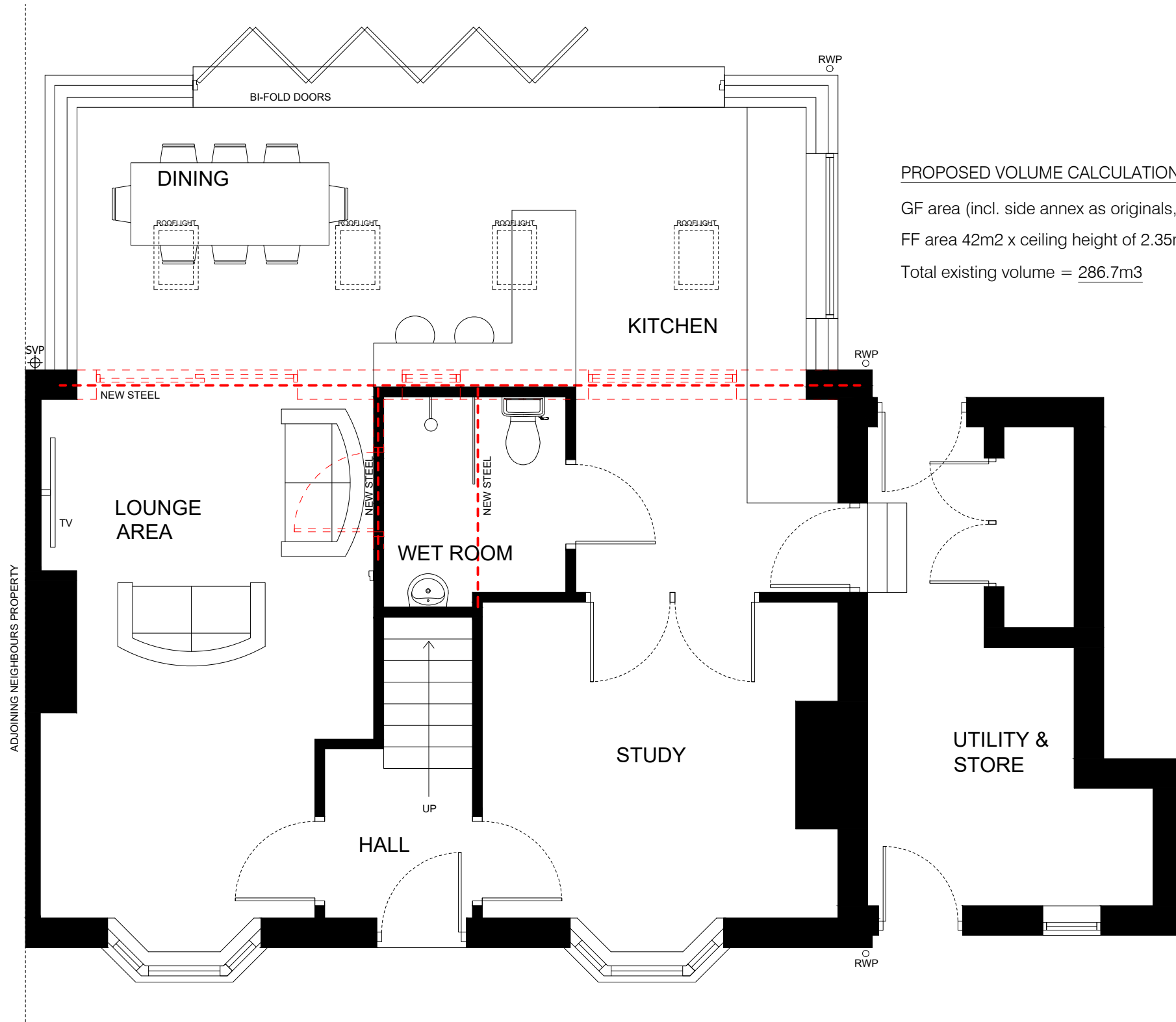
PROPOSED GROUND FLOOR PLAN - 66m 2
