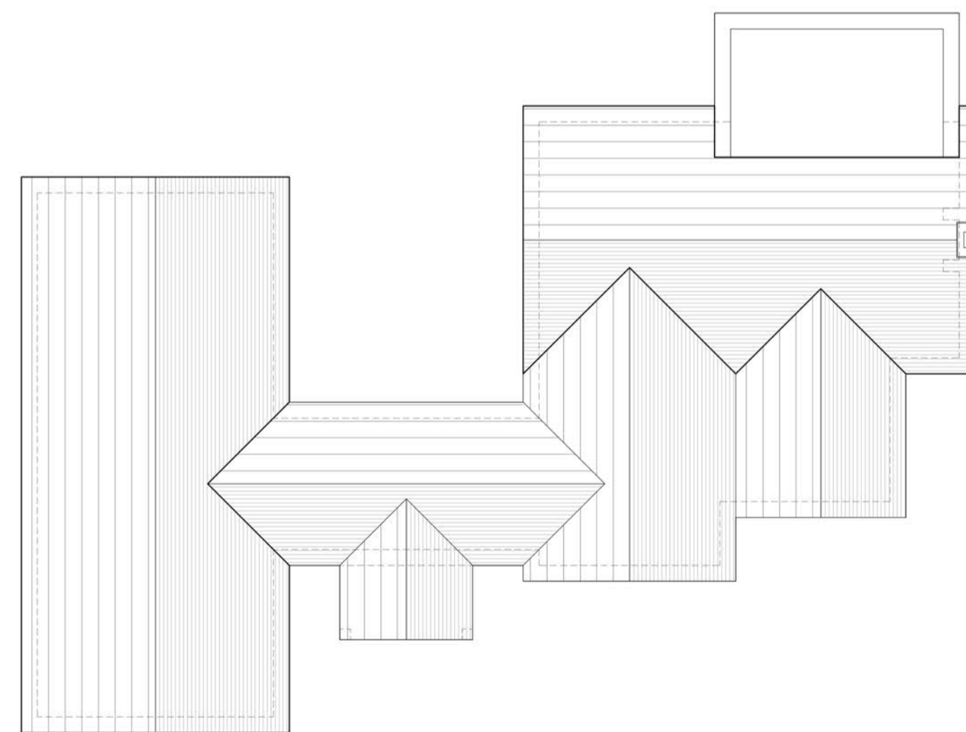
Roof Plan
