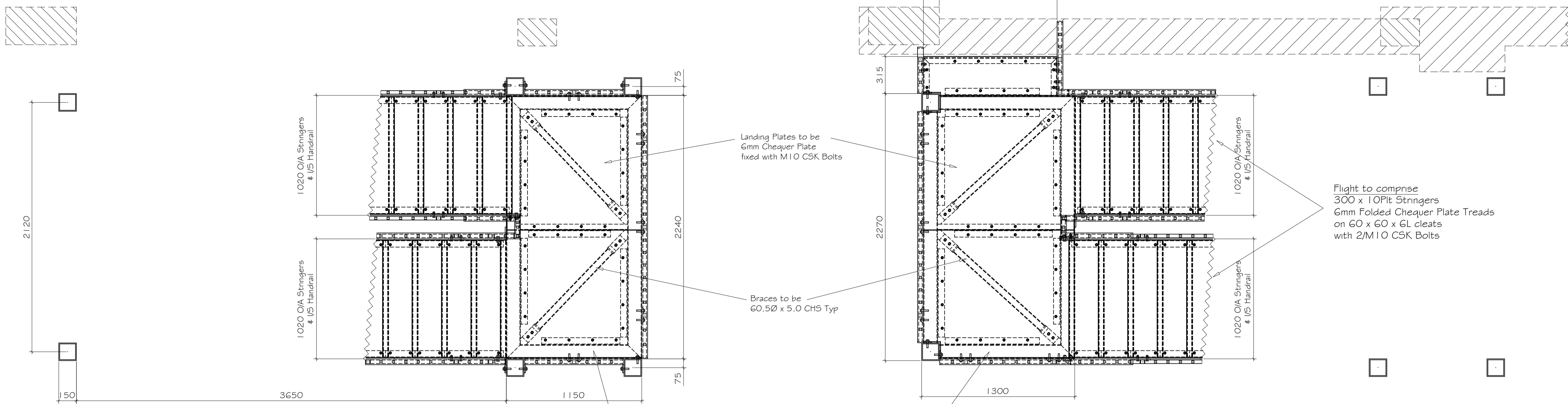
Plan View Half Landing Ground to 1st Floor 1:20
