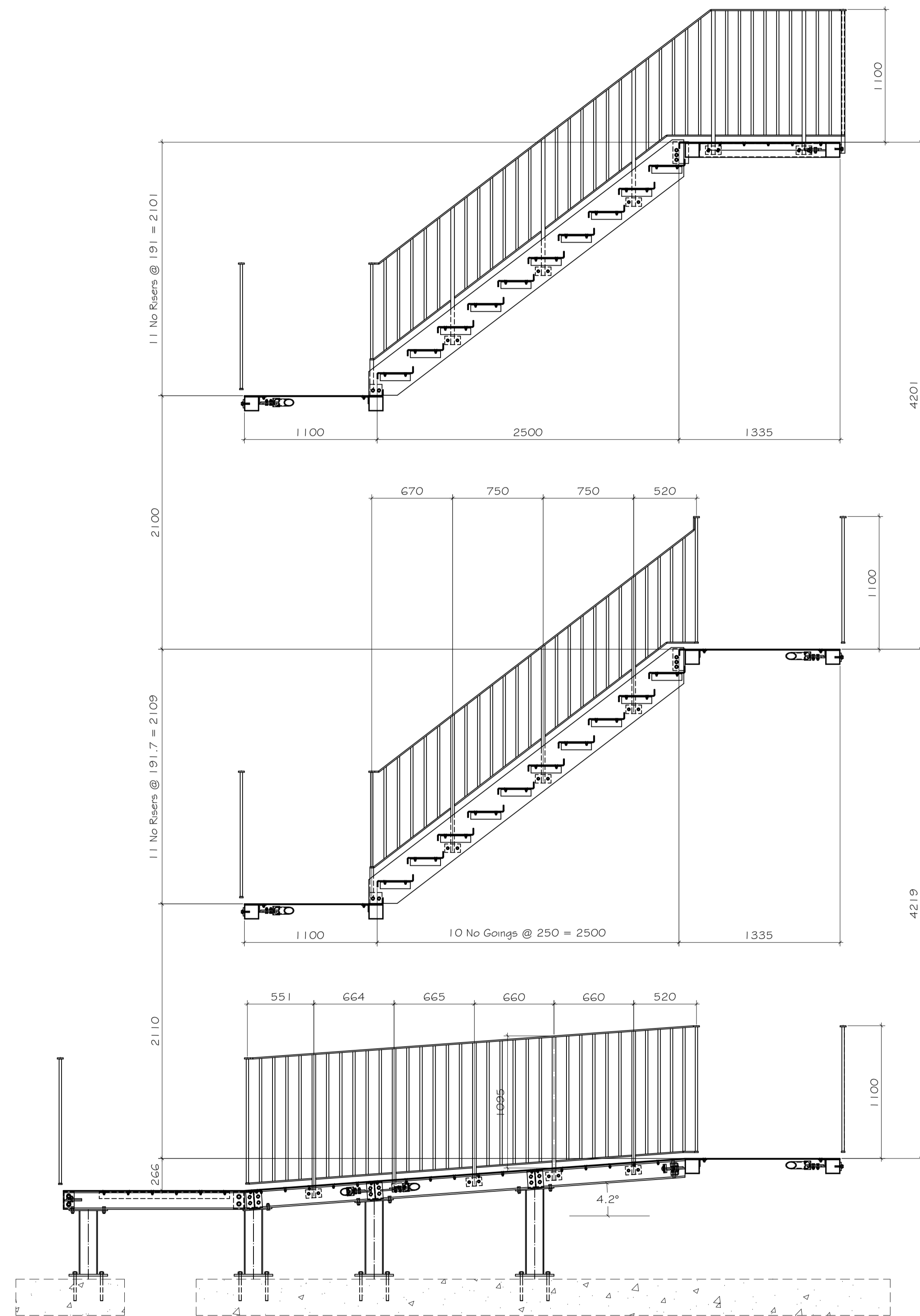
Section B-B 1:25
