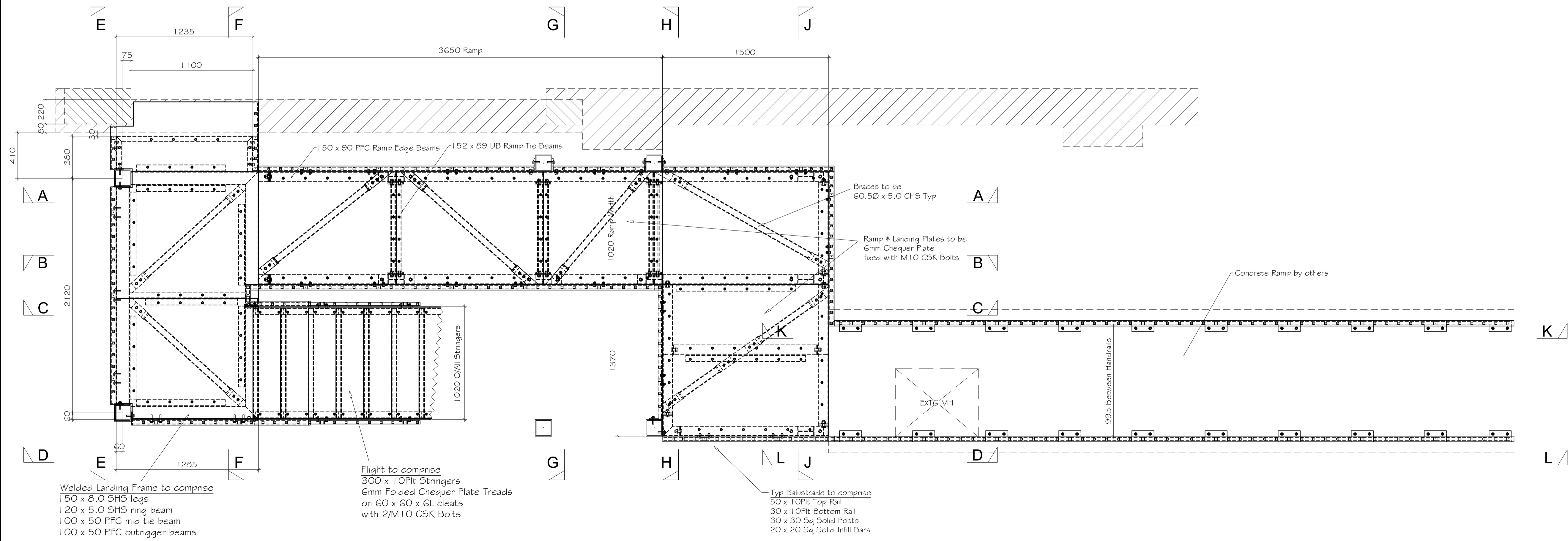
Plan View Ramp & Ground Floor Level 1:20
