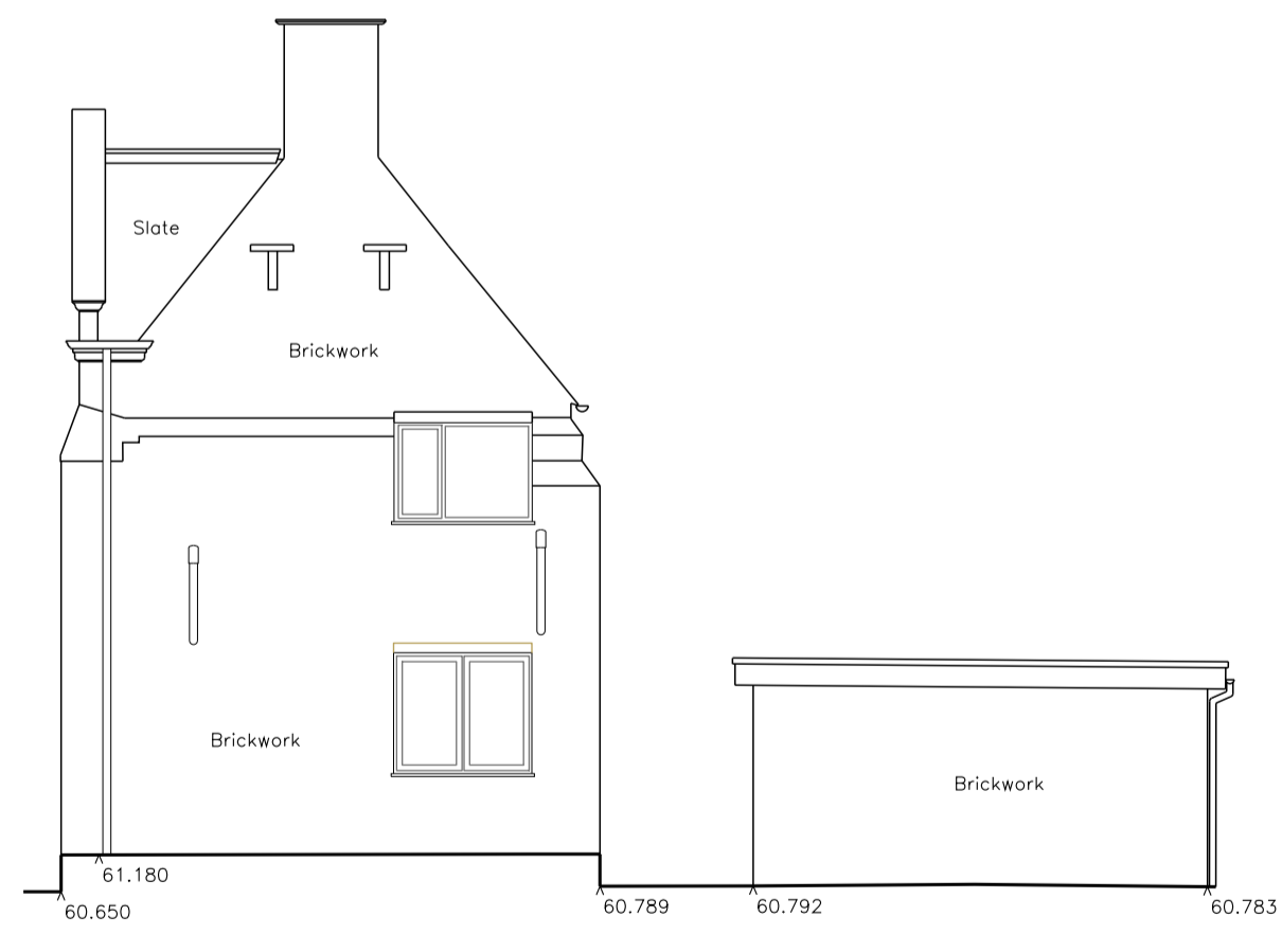
1911 Classroom Block - North Elevation to Sub-Station
