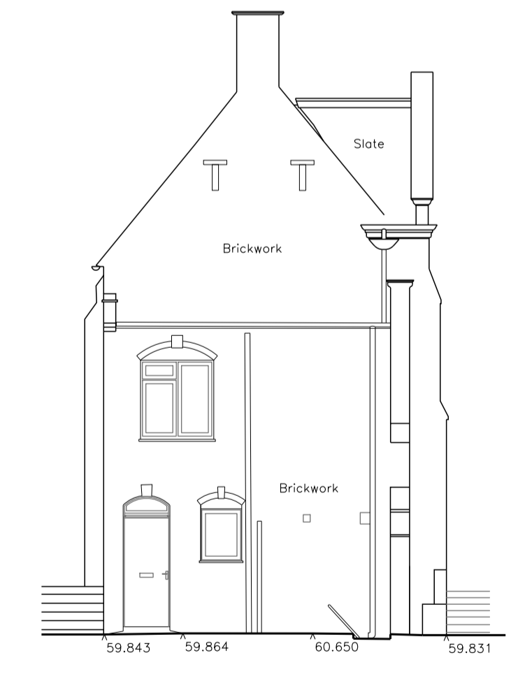
1911 Classroom Block South Facing Elevation
