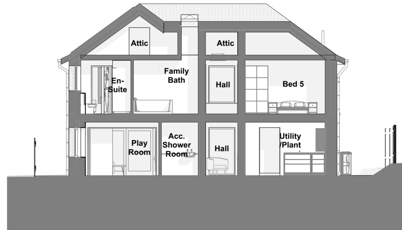
B Typical Cross Section 1:100
