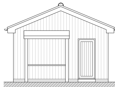
SIDE / NORTHERN ELEVATION
