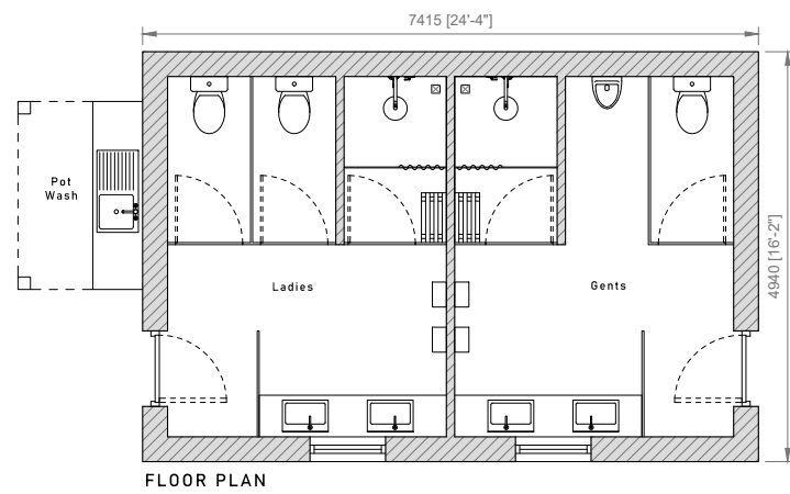
FLOOR PLAN
