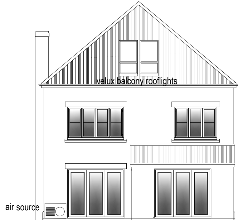
Proposed Rear Elevation (southeast)
