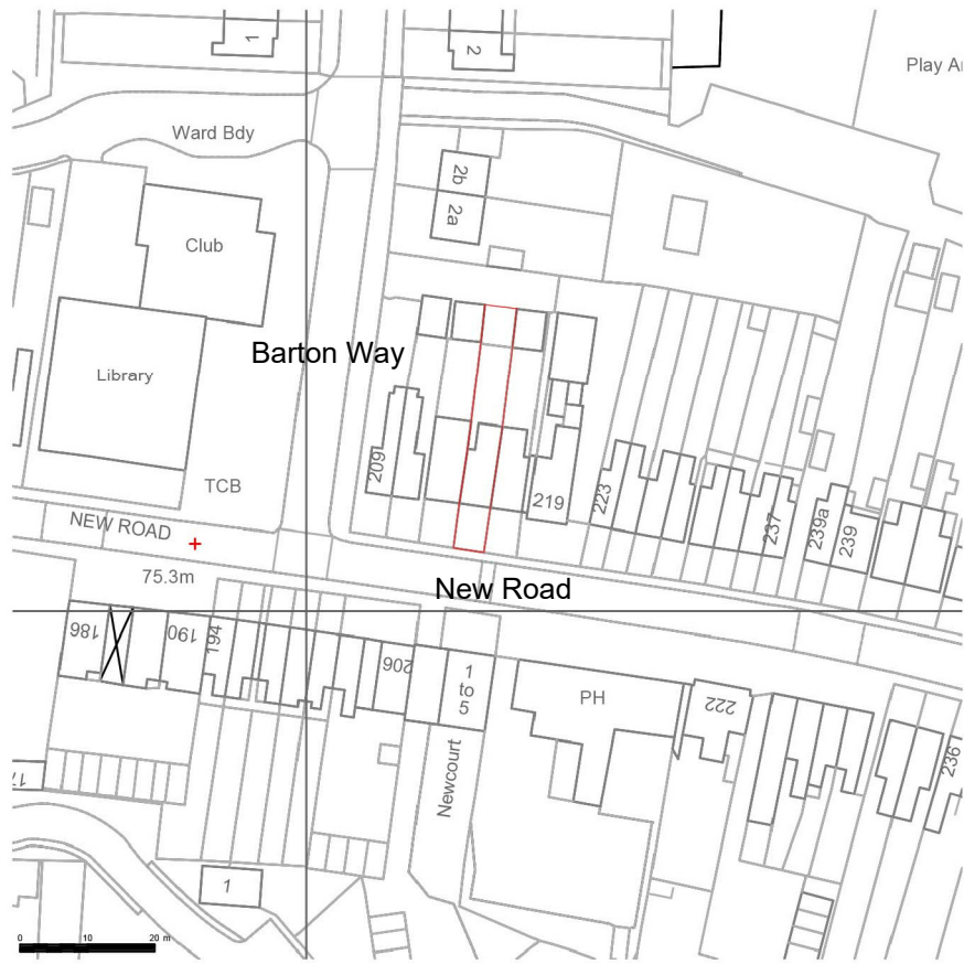
Site Location Plan Scale 1:1250 @ A4
