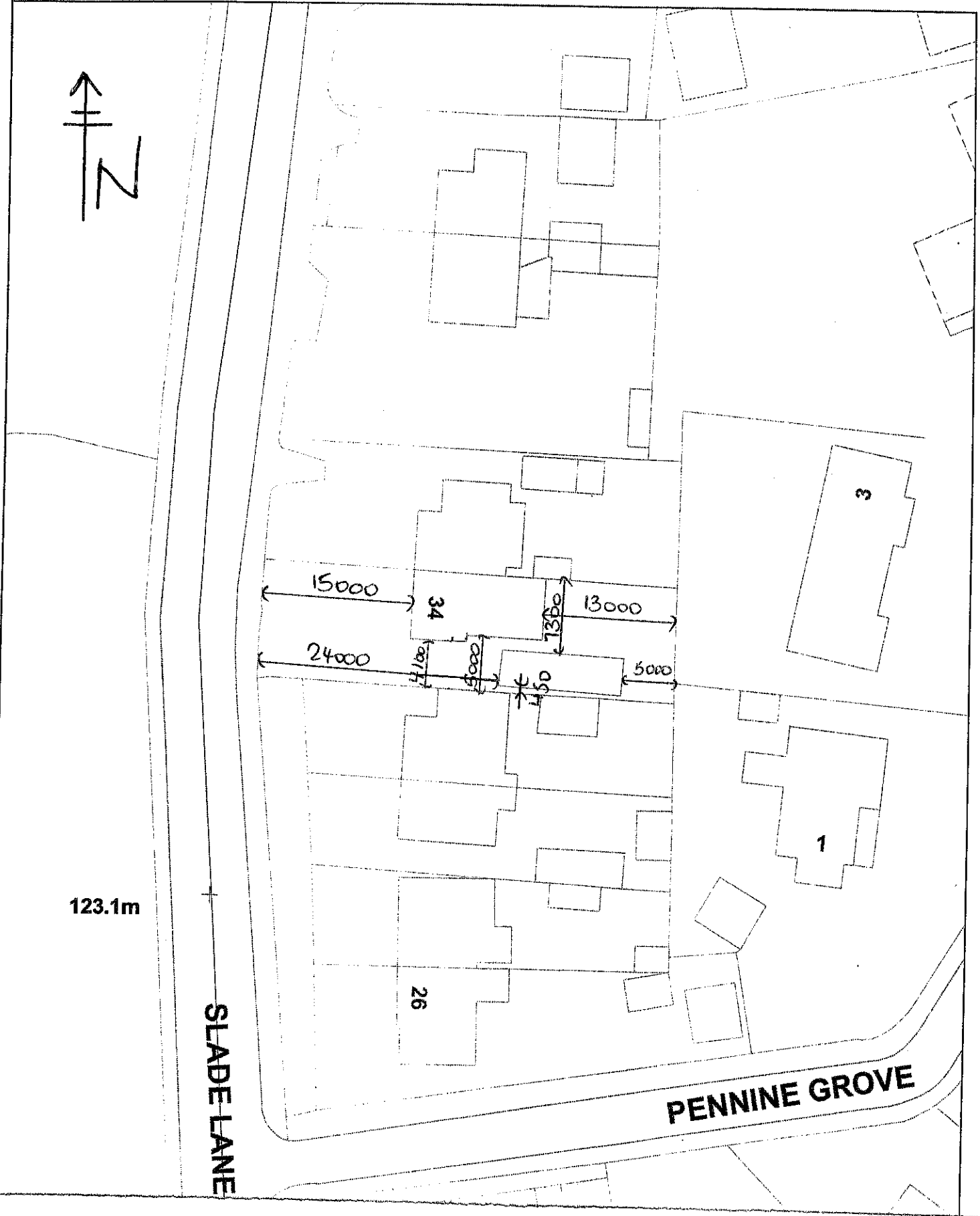
EXISTING SITE PLAN 1:500 DRWG S.L34/H
