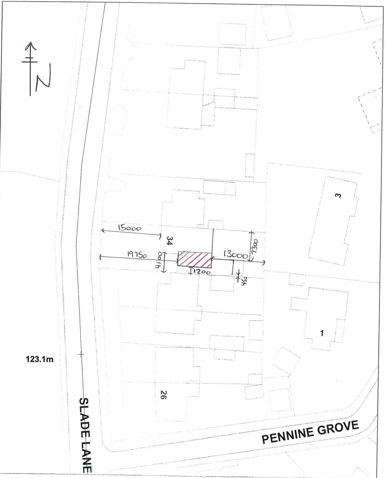
PROPOSED SITE PLAN 1:500 DRWG: S.L 34 / 5
