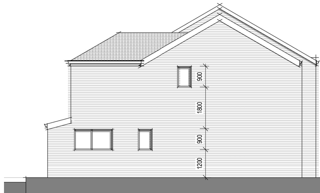
Side Elevation 1 : 100
