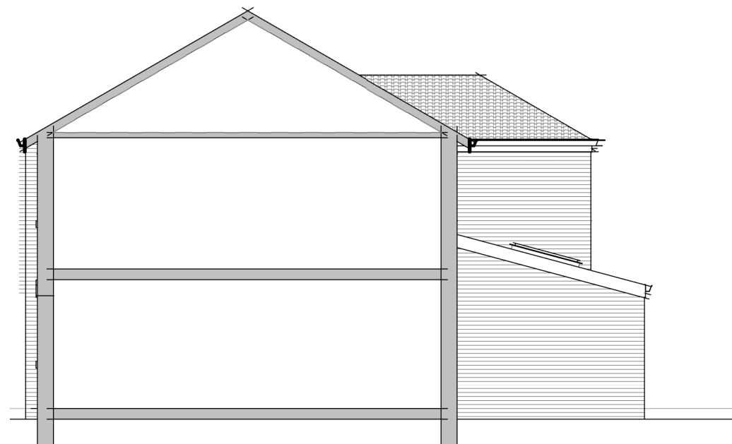
Side Elevation from Adjacent Plot 1 : 100
