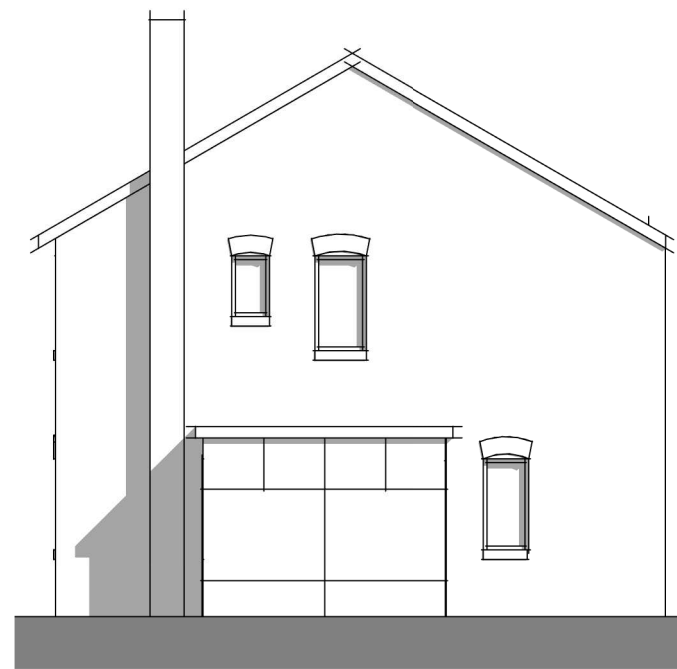
Side Elevation 1 : 100
