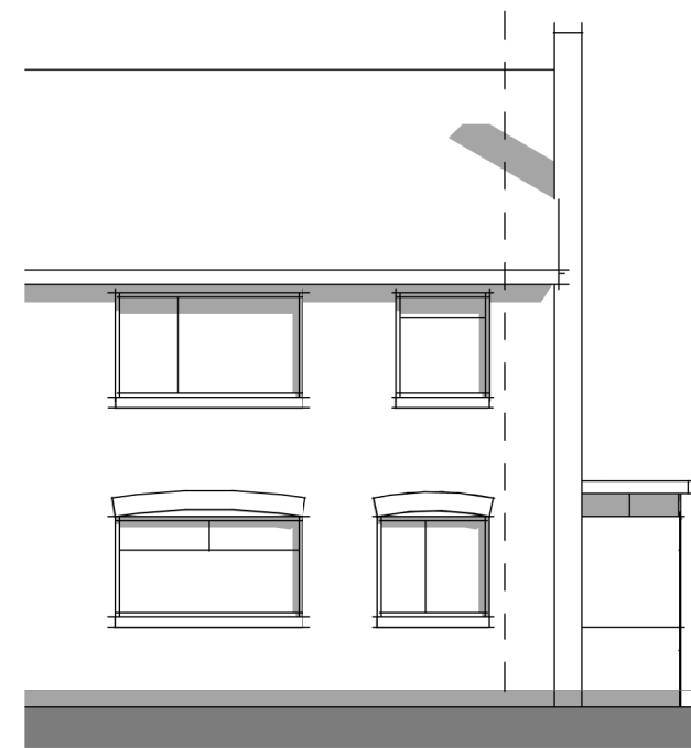
Rear Elevation 1 : 100
