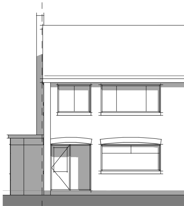
Front Elevation 1 : 100
