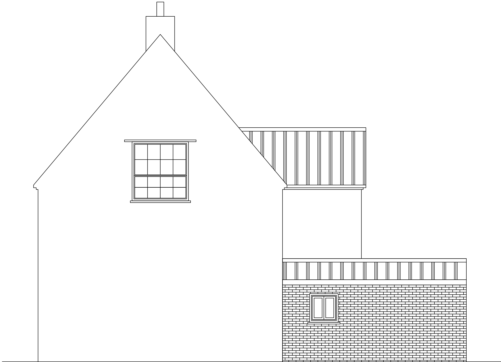
SIDE ELEVATION EXISTING 1:50
