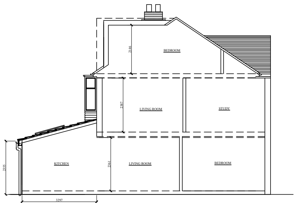
SECTION VIEW A-A (APPROVED)
