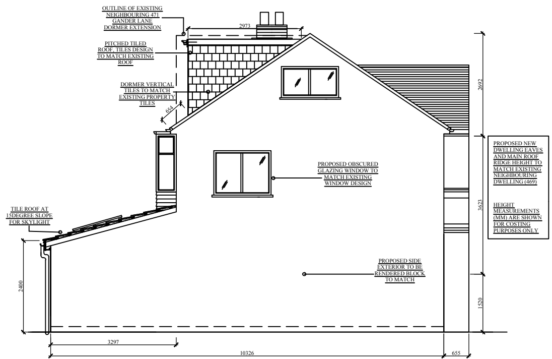
SIDE ELEVATION (APPROVED)
