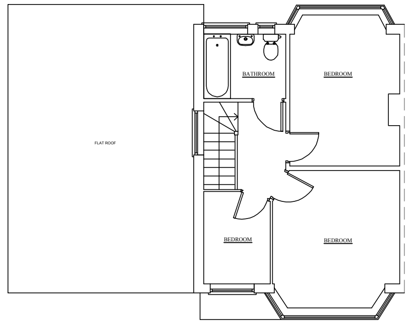
FIRST FLOOR PLAN (PRE-EXISTING)
