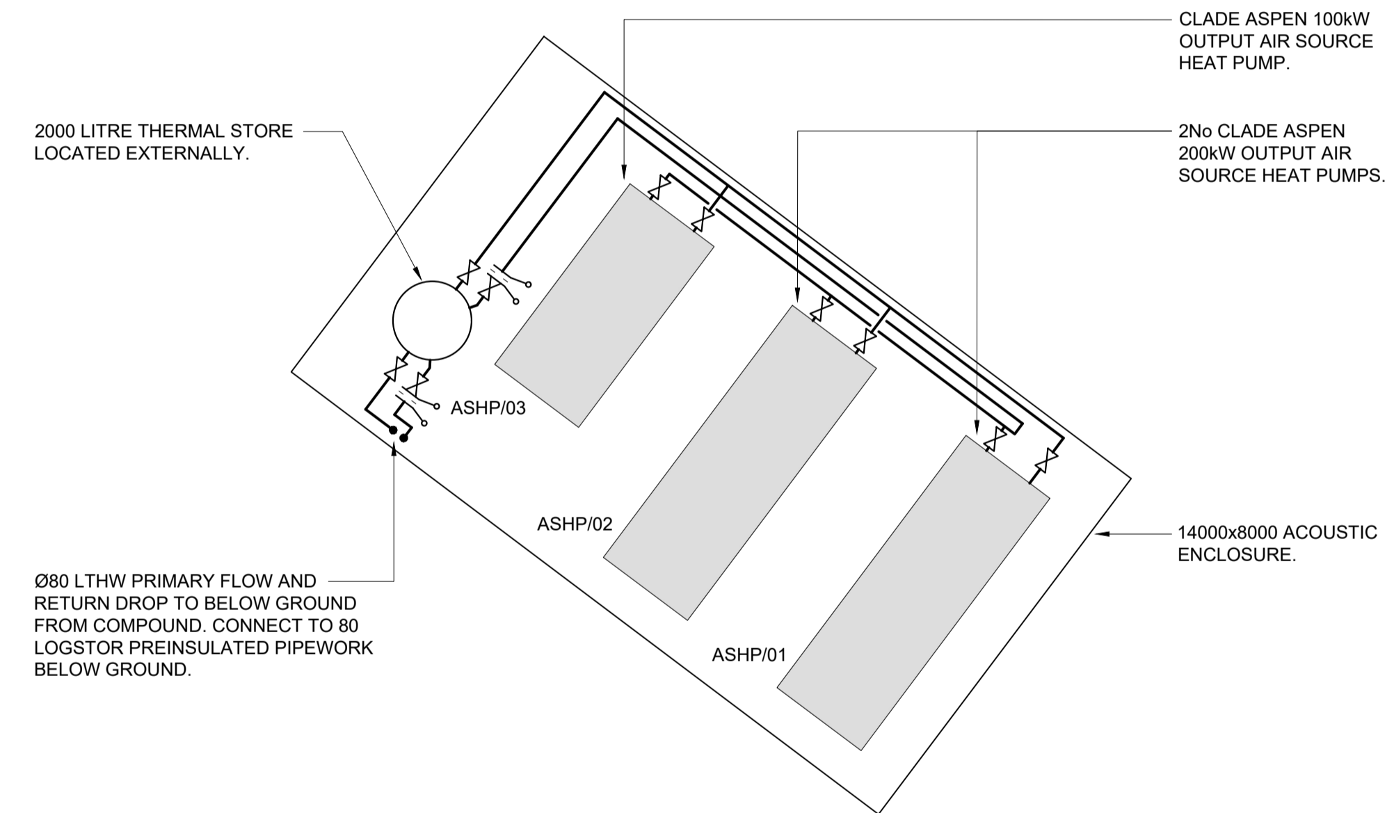
DETAIL A: ASHP COMPOUND LAYOUT
