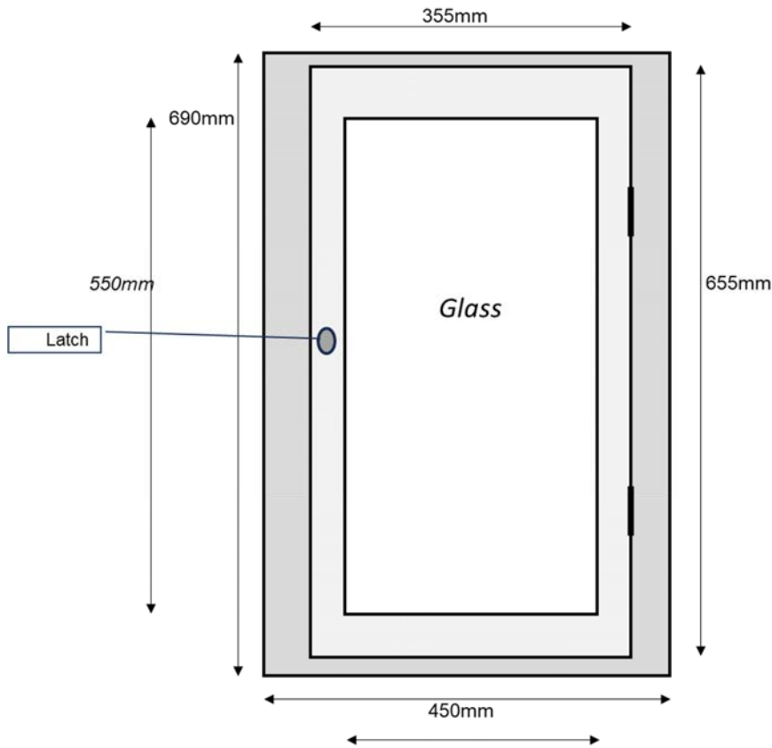
Figure 2 - Diagram of window to be replaced
