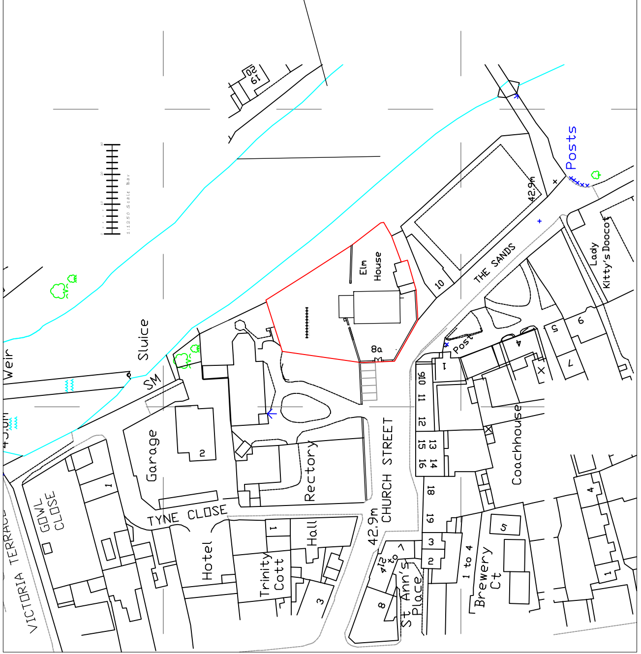
Block Plan Scale 1:250
