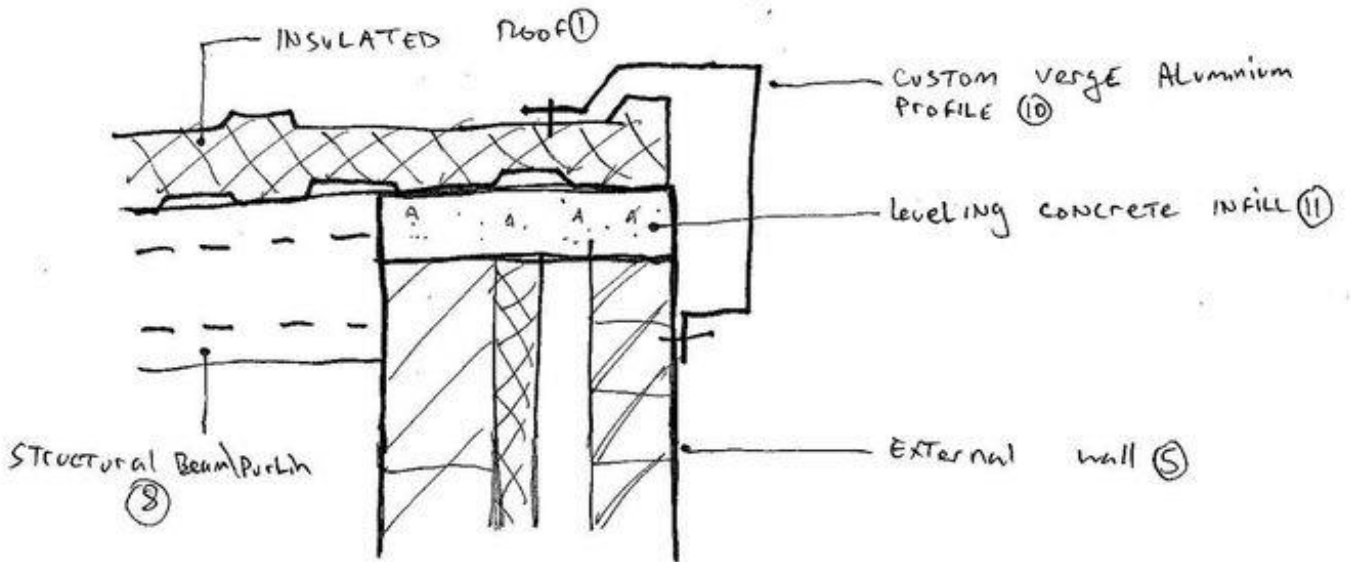
SECTION 2 - VERGE DETAIL
