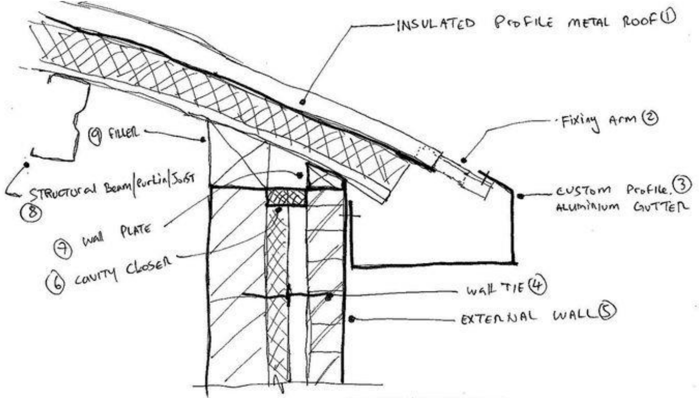
SECTION 1 - GUTTER/EAVES
