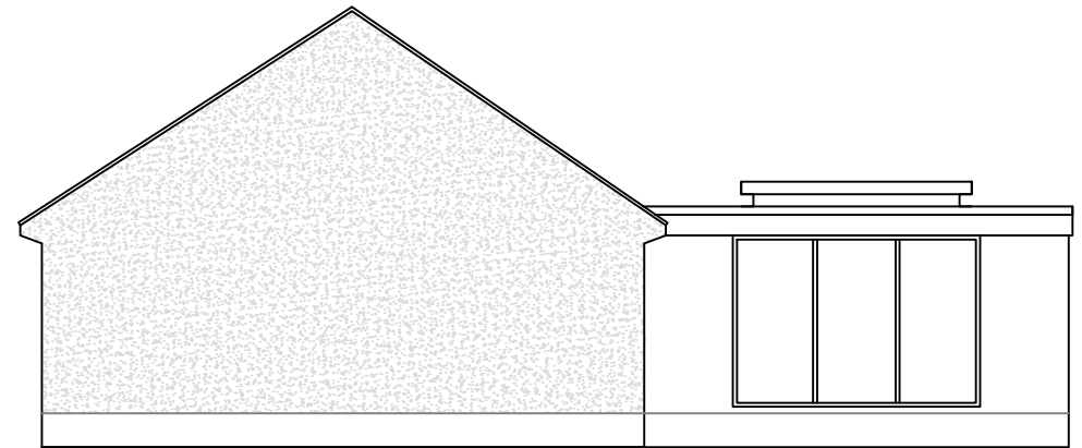
Proposed Side (NE) Elevation
