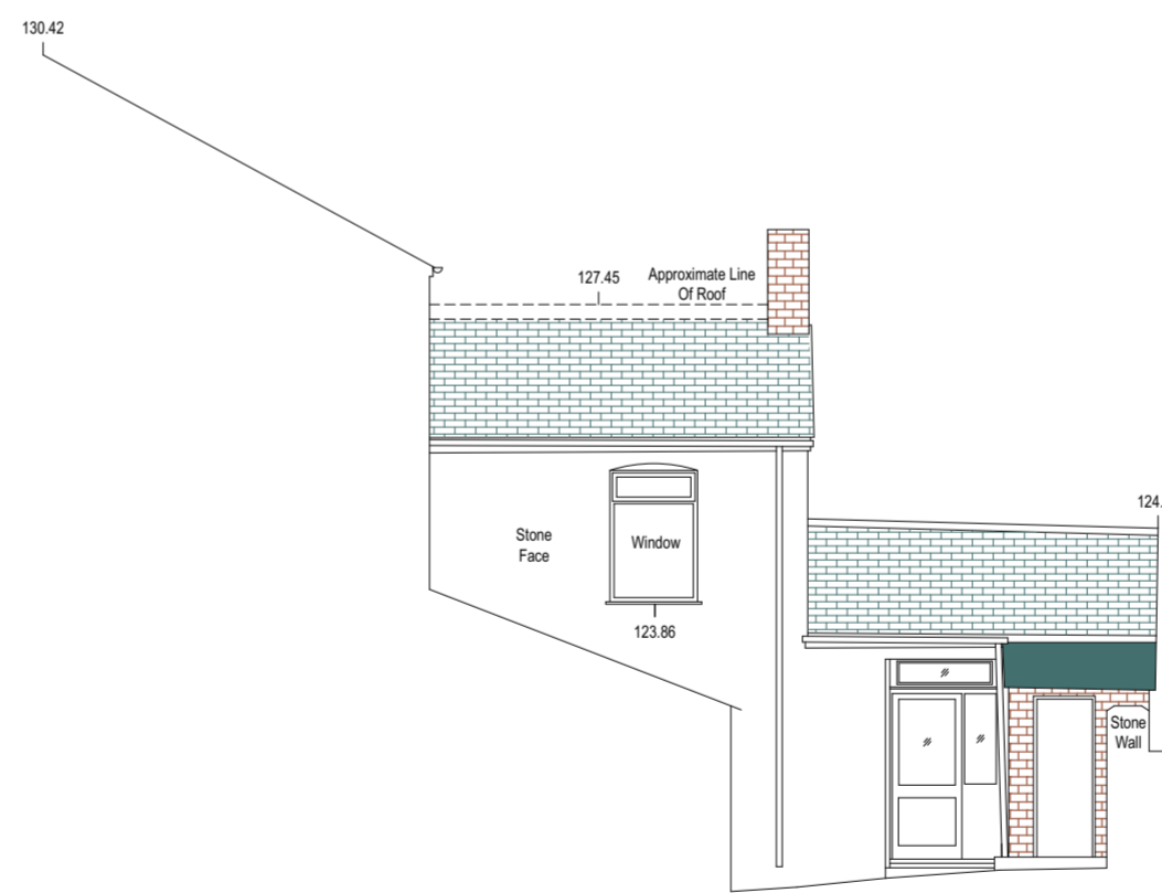
Datum 115.00m South East Elevation
