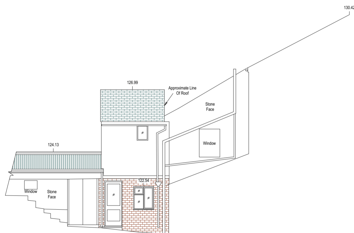
Datum 115.00m North West Elevation
