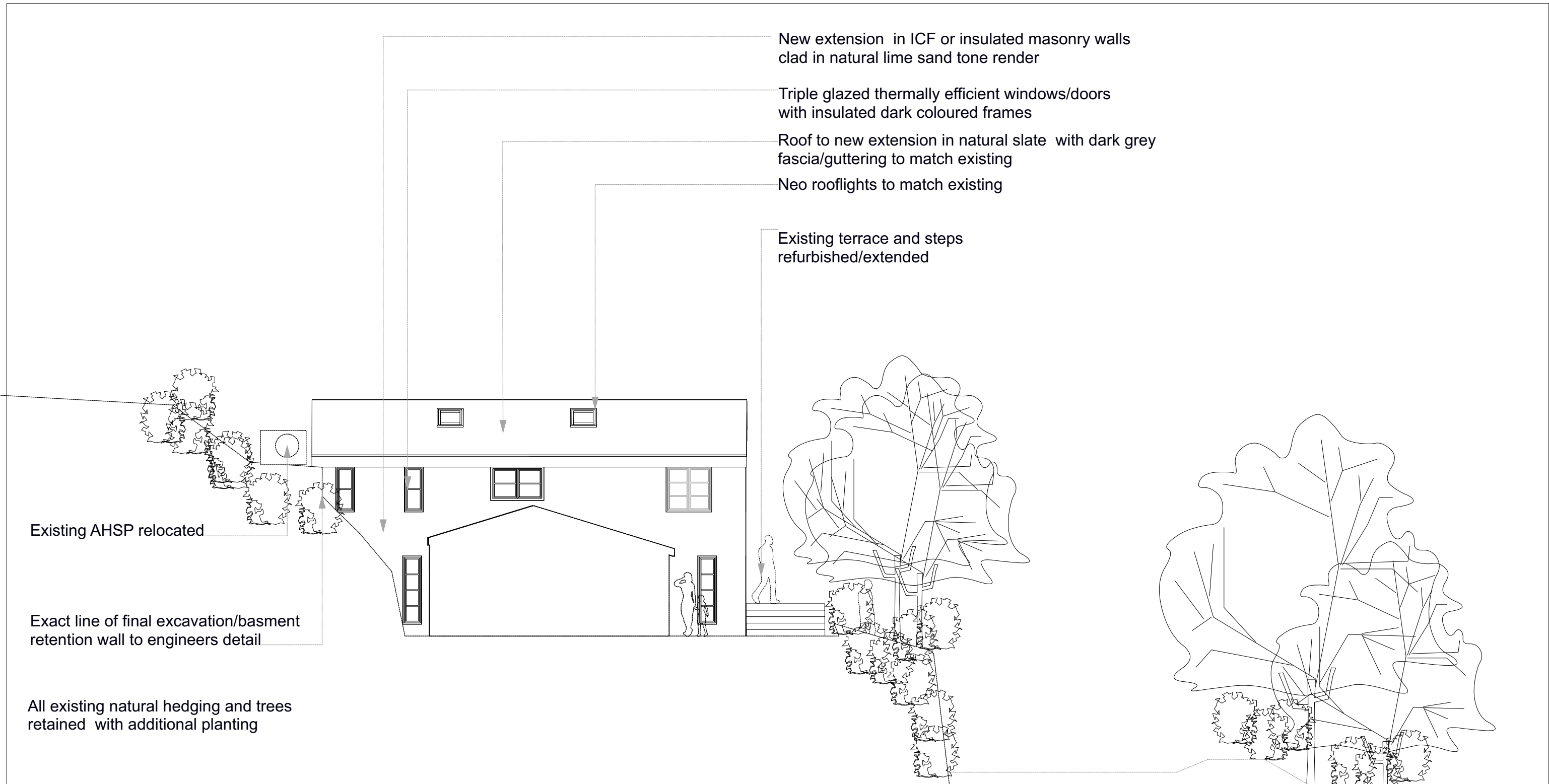
AA Extension west elevation Scale: 1:100
