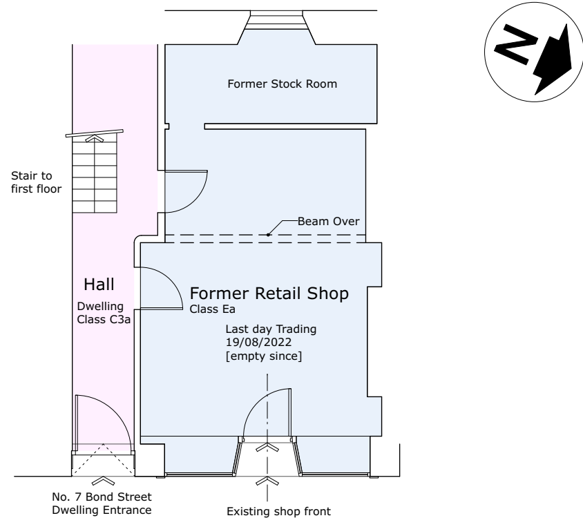
Existing Floor Plan 'Harveys' [Former Newsagents / Tobacconists] 7, Bond Street Redruth
