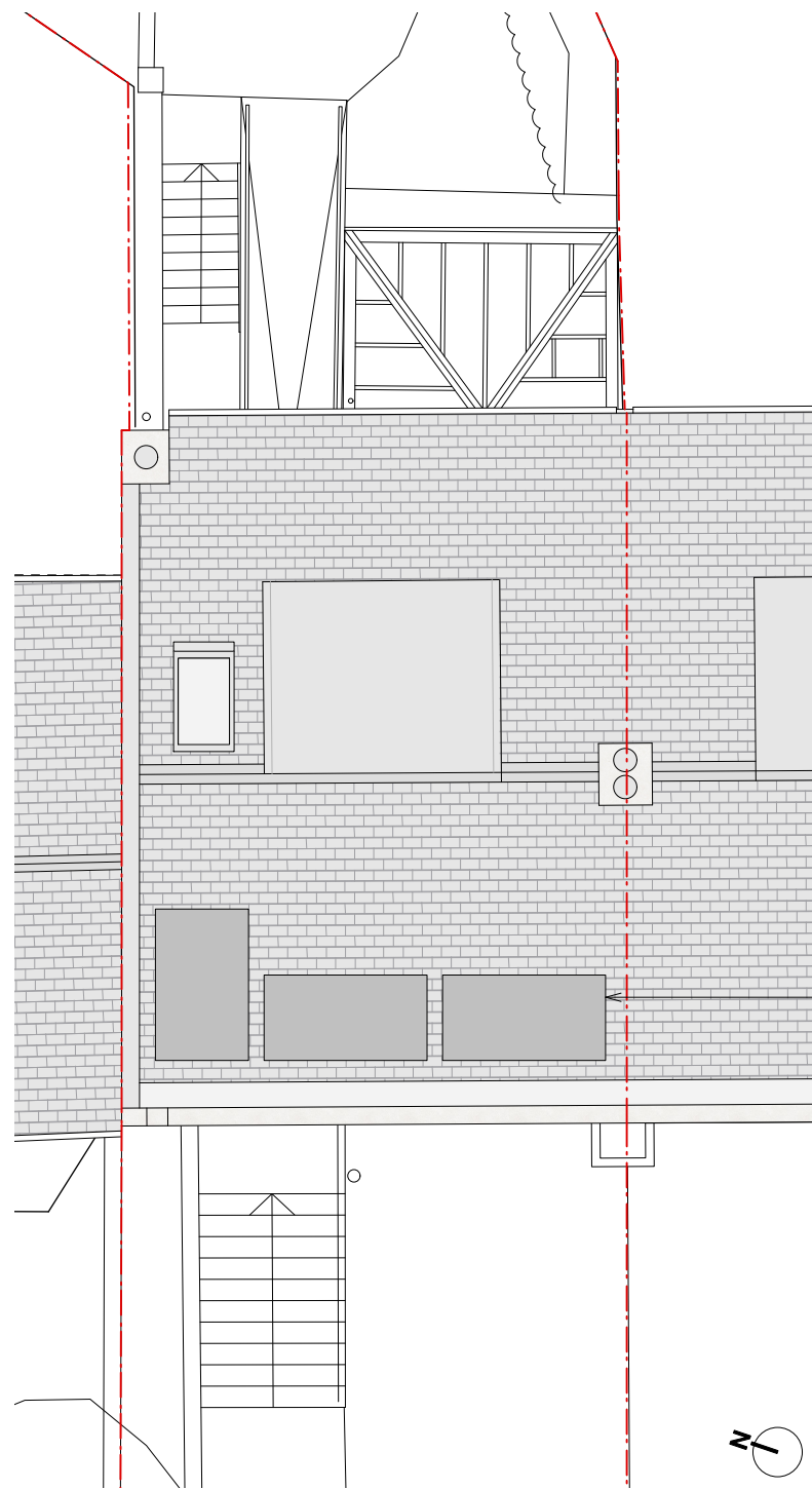
1 Proposed Roof Plan
