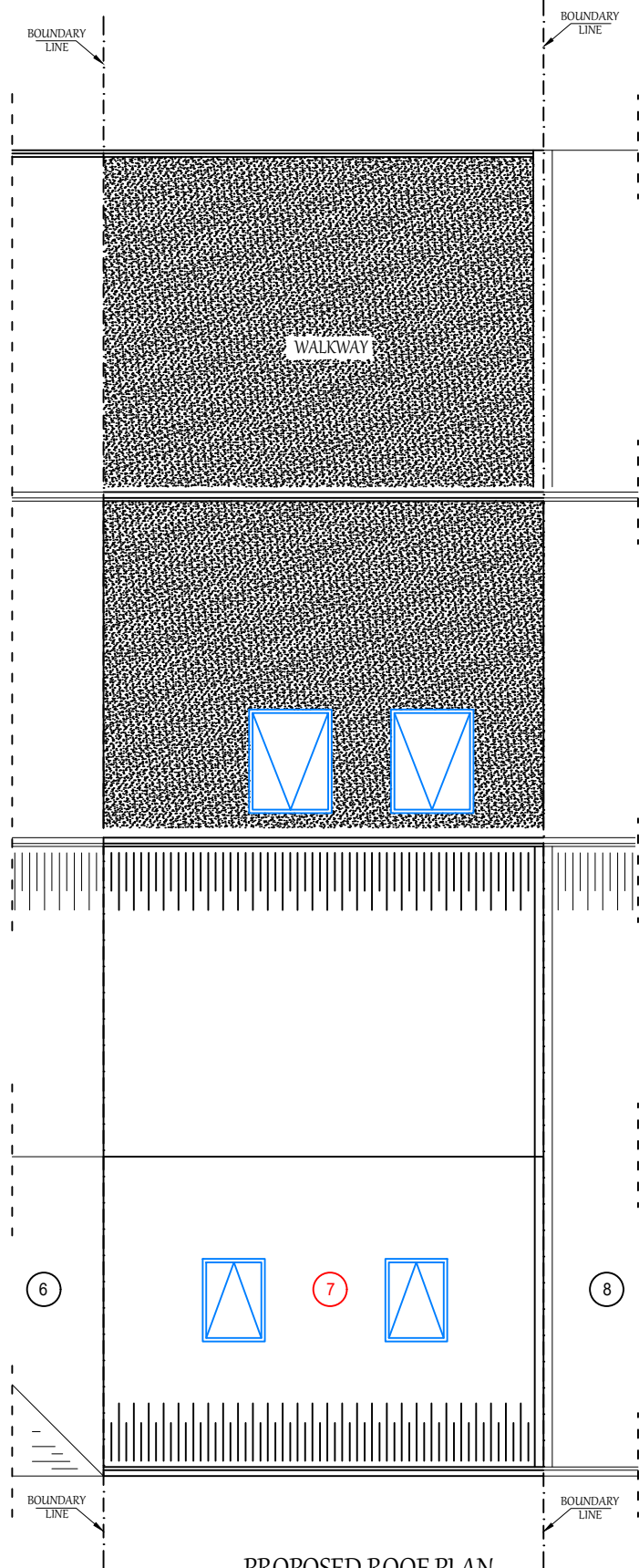
PROPOSED ROOF PLAN SCALE: 1/100 @A3
