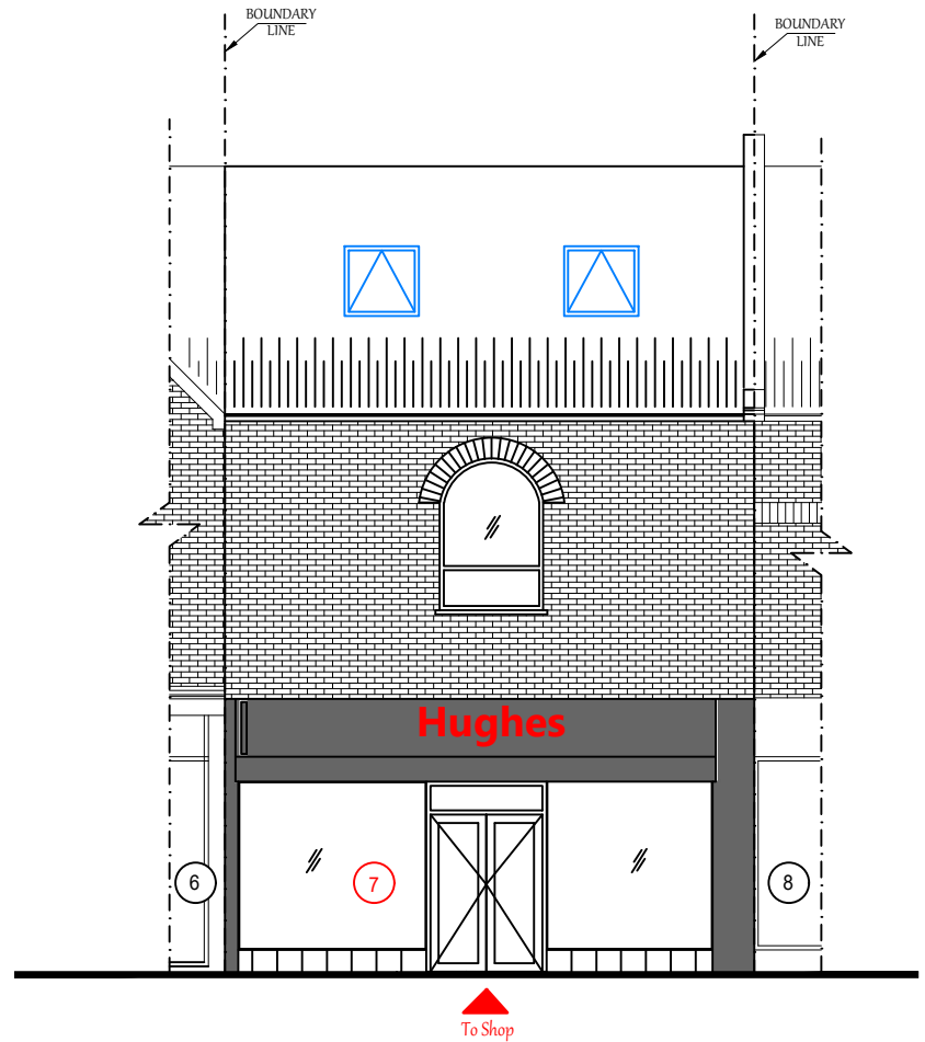
PROPOSED FRONT ELEVATION SCALE: 1/100 @A3
