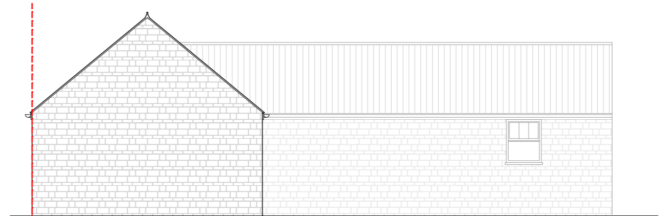
Front Elevation
