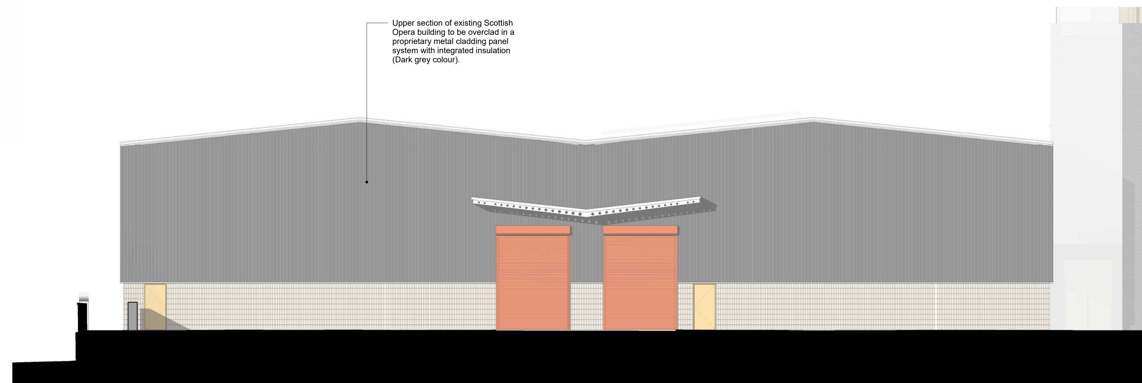
Proposed elevation - Existing S.O. building (South)
